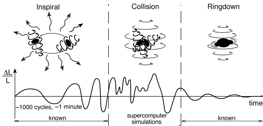
Fig. 5.16. Inspiral and merger of two black holes
