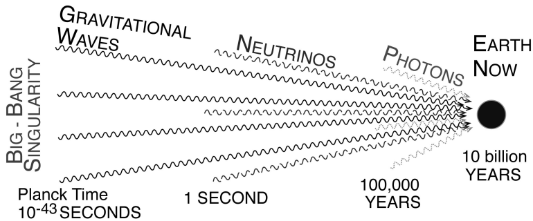
Fig. 5.19. Unlike photons and neutrinos, only gravitational waves can look back to the earliest moments of the universe
