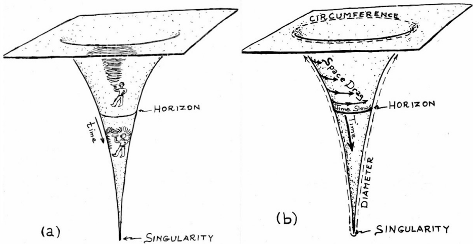
Fig. 5.5. (a) Kip falling into a black hole and trying to transmit microwave signals to you on the outside. (b) The curvature of space, the warping of time, and the dragging of space into a tornado-like motion around a spinning black hole.
