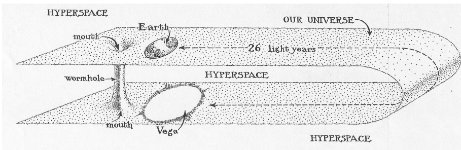
Fig. 5.23. A hypothetical wormhole connecting our solar system to the vicinity of the star Vega. [From my book Black Holes and Time Warps: Einstein's Outrageous Legacy (W.W. Norton, New York, 1994).]
