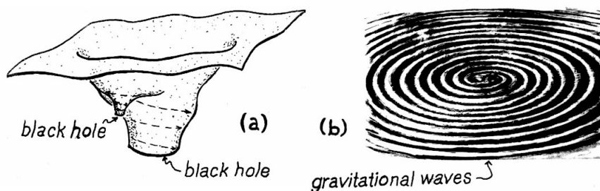
Fig. 5.7. Left: a small black hole orbiting a large black hole and gradually spiraling inward. Right: the gravitational waves produced by the small hole's inspiral.
