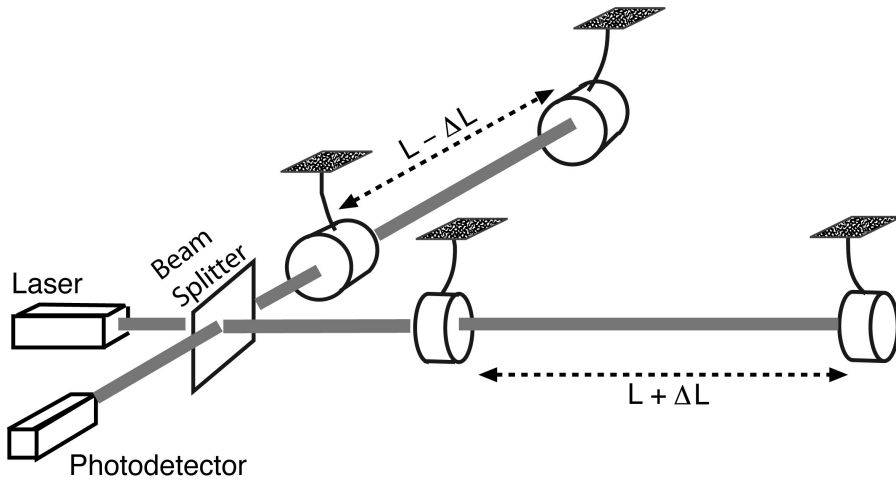
Fig. 5.15. Sketch of an earth-based gravitational-wave interferometer
