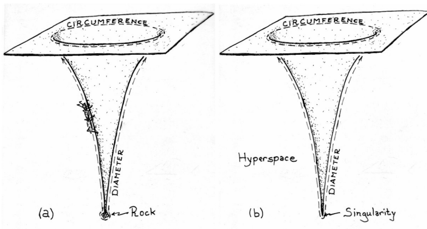
Fig. 5.4. A rubber sheet warped by a heavy stone (left) is an excellent analogy for a black hole's warped space (right).
