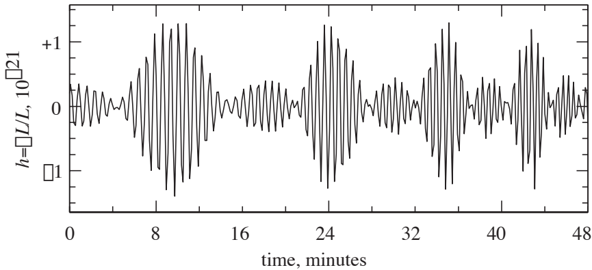
Fig. 5.11. The gravitational waveform passing LISA shortly before the small hole reaches the end of its inspiral and begins a catastrophic plunge into the big hole’s horizon. This waveform was computed by Scott Hughes, a former student of mine, by solving Einstein’s general relativity equations. LISA is assumed to be in the equatorial plane of the big hole, and the small hole’s orbit is inclined 40 degrees to that plane.
