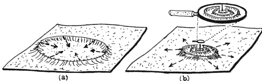
Fig. 5.22. The supercomputer simulations of imploding waves, which triggered Hawking to concede that the laws of physics permit naked singularities, at least in principle.
