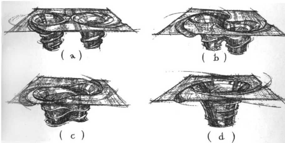
Fig. 5.13. The collision and merger of two black holes: an artist's conception. [Courtesy the LIGO Project, California Institute of Technology.]
