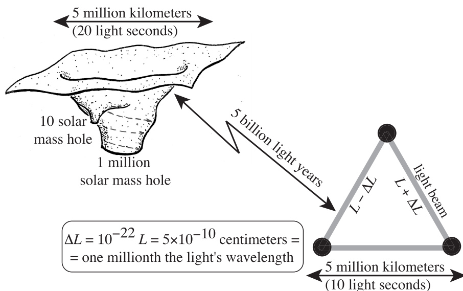
Fig. 5.10. Some numbers for LISA's bothrodesy mapping of a massive black hole.
