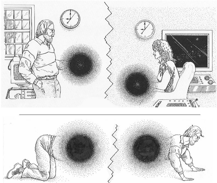
Fig. 5.24. Time travel. [Adapted from my book Black Holes and Time Warps: Einstein's Outrageous Legacy (W.W. Norton, New York, 1994).]
