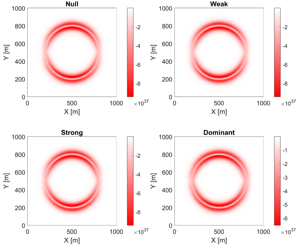
Figure 4. Energy condition evaluation for the Alcubierre metric. The motion of the bubble is in the +X . The slice is for z = z_0 , v_s = 0.1 c, R = 300 m, \sigma = 0.015 \text{ m}^{-1} , x_0 = y_0 = z_0 = 503 m, n_{\text{observers}} = 1000 . The minimum value among all observers is shown. Units are in \text{J m}^{-3} .
