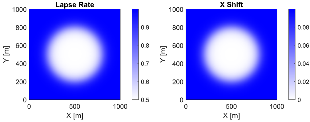
Figure 11. Metric components for the comoving modified time metric. The motion of the bubble is in the +X direction. The slice is for z = z_0 , v_s = 0.1 c , A_{\max} = 2 , R = 300 m, \sigma = 0.015 \text{ m}^{-1} , x_0 = y_0 = z_0 = 503 m.
