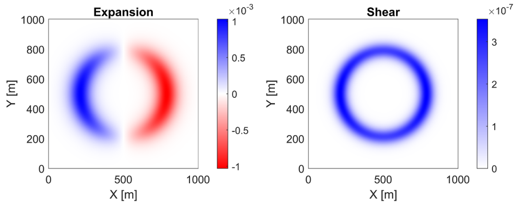
Figure 15. Expansion and shear scalars for the modified time metric. The motion of the bubble is in the +X direction. The slice is for z = z_0 , v_s = 0.1 c , A_{\max} = 2 , R = 300 m, \sigma = 0.015 \text{ m}^{-1} , x_0 = y_0 = z_0 = 503 m.
