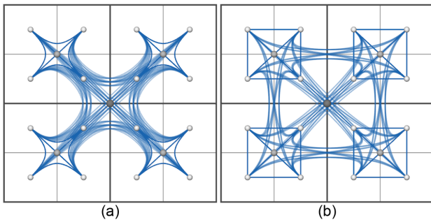
Fig. 6. Removing the LCA from the original control polygon. A tree of depth 2 and its additional adjacency graph ( \beta = 0.85 ) visualized as a treemap with (a) LCA present, and (b) LCA removed. LCA removal effectively prevents connections between sibling nodes from curving toward their common parent node.
