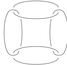
Figure 9: A link in S^3
