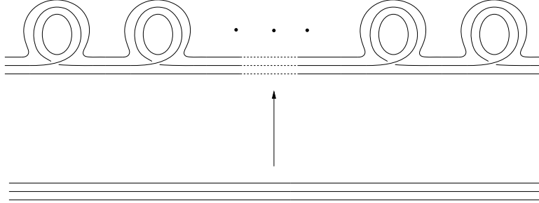
Figure 20: Adding some curls along an edge of a special polyhedron.
