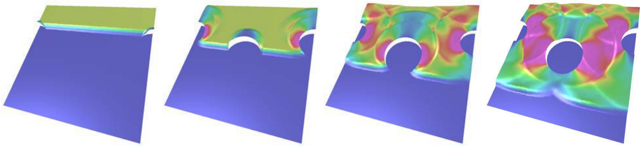
Figure 7: Shock passing through a medium with circular inclusions. The shock causes the inclusions to debond from the surrounding medium.
