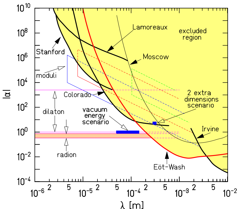
Figure 1: Regions in the \alpha - \lambda plane excluded by table top searches for deviations from Newtonian gravity from Adelberger et al. [12]. The ADD prediction with n = 2 and M_* = 1 TeV is also shown.
