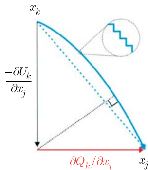
Figure 2. Flow of energy directs from the high potential U_k at x_k down along the geodesic of space–time towards the low potential U_j at x_j . The gradient -\partial U_k / \partial x_j (black vertical arrow) translates invariant mass m_k into acceleration a_k along the steepest gradient (blue arrow). The directed arc \mathbf{s} is curved owing to the concurrent dissipation \partial Q_k / \partial x_j (red horizontal arrow) that stems from the differences in interactions that distinguishes the state k from j . The curvilinear motion adds up (equations (4.3) and (4.4)) from the potential gradient and dissipative projections. The chord (dashed line) is a good approximation of \mathbf{s} in a locality that does not curve much. The expanded microscopic path forms from quantized actions.
