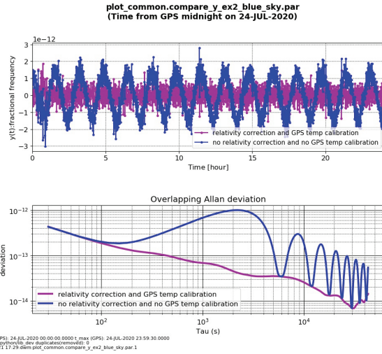
Figure 7: Top plot shows y(t) before relativity correction and GPS temperature calibration in blue and y(t) after relativity correction and GPS temperature calibration in magenta for a single day of data. A frequency bias has been removed from the y(t) data. Orbital variations primarily due to relativistic effects are clearly seen in the blue y(t) data. Bottom plot shows the corresponding Allan deviations which are the standard way to represent clock stability for different timescales \tau .
