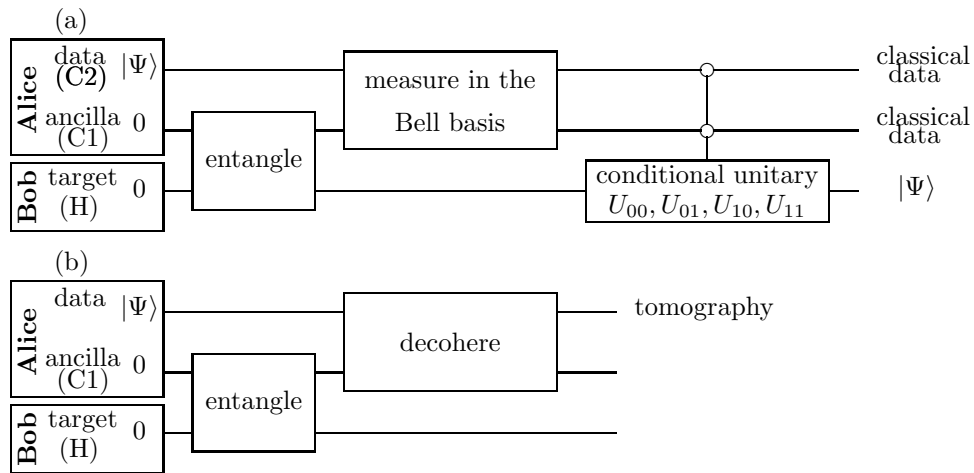
Figure 1: Schematic circuits for (a) the quantum teleportation experiment, and (b) the control experiment. The teleportation circuit is based upon that suggested by Brassard et al 21 . Note that the control circuit simply omits two elements of the teleportation experiment – rotation from the Bell basis into the computational basis, immediately before the decoherence step, and the conditional unitary operation. Commented pulse sequences for our experiment may be obtained on the world wide web 13 .
