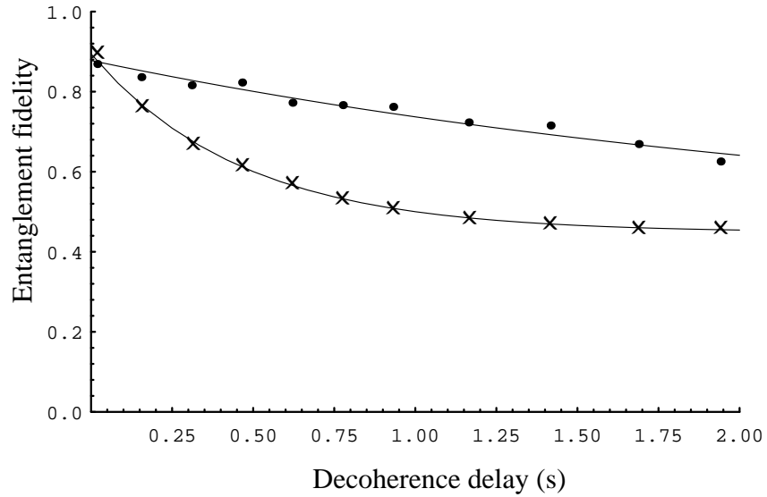
Figure 2: Entanglement fidelity (a measure of how well quantum information is preserved) is plotted as a function of decoherence time. The bottom curve is a control run where the information remains in C2. The curve shows a decay time of approximately 0.5s. The top curve represents the fidelity of the quantum teleportation process. The decay time is approximately 2.6s. The information is preserved for a longer time, corresponding approximately to the combined effects of decoherence and relaxation for the Hydrogen, confirming the prediction of teleportation.
