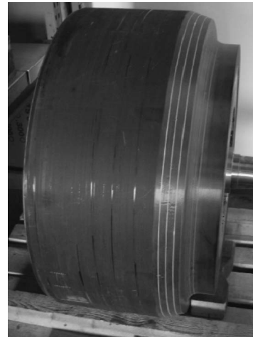
Fig. 3. Multirim flywheel rotor.
