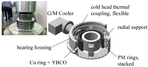
Fig. 4. Schematics of the HTS bearing structure with cold head. The insert shows part of the assembled PM rotor.
