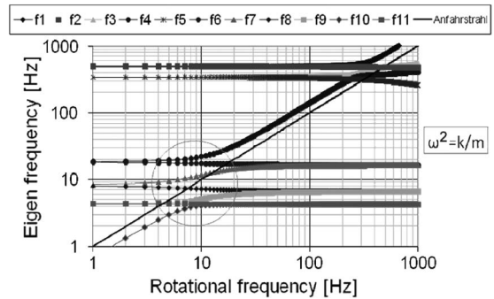
Fig. 5. Calculated diagram of flywheel rotor eigenfrequencies.
