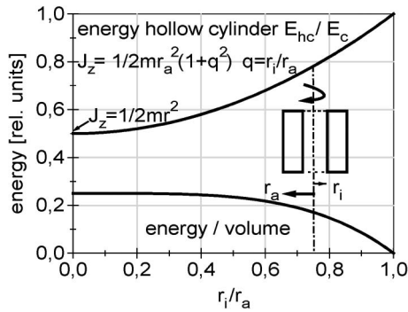
Fig. 7. Geometry and energy factors of a rotating hollow cylinder.
