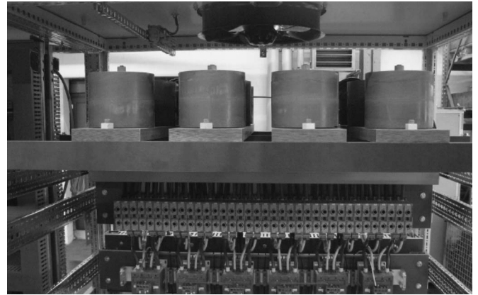
Fig. 6. Power distribution unit of the 5-kWh HTS FESS.
