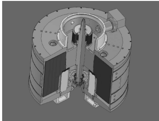
Fig. 2. HTS flywheel inner structure.
