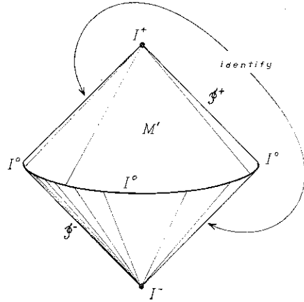
Fig. 1. Compactified Minkowski space $M$. $I^0, I^+, I^-$ are points at spatial infinity, future time infinity and past time infinity respectively, while $\tilde{I}^+, \tilde{I}^-$ are future and past null infinity cones (cf. [3]). The compactified space has $I^0, I^+, I^-$ identified and $\tilde{I}^-, \tilde{I}^+$ identified along opposite generators. For typographical reasons, "$I$" replaces the more usual script $I$ depicted in figs. 1 and 40.
