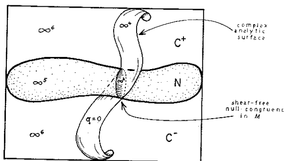
Fig. 4. The Kerr theorem.
