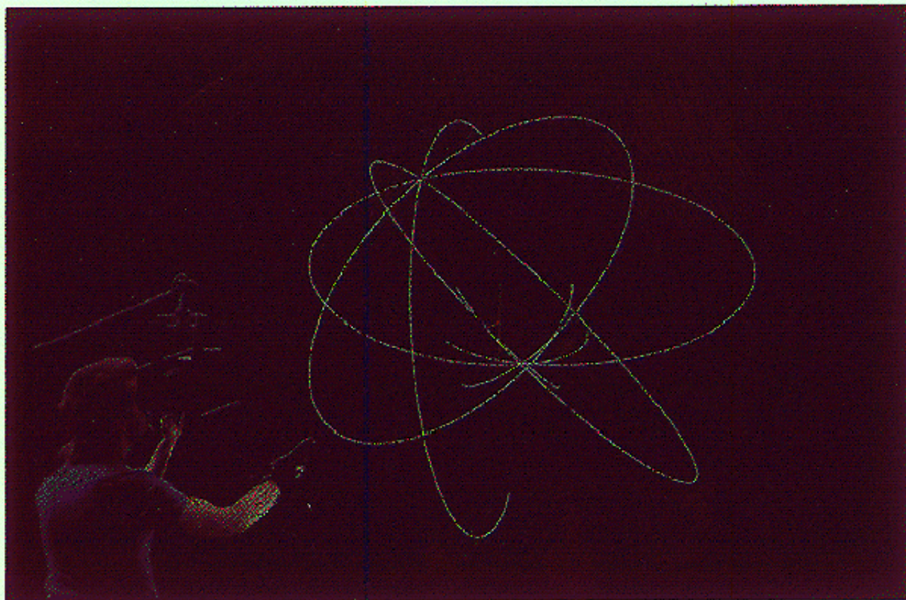
Figure 1: The virtual spacetime system in use, showing the manipulation and observation of a spray of geodesics.
