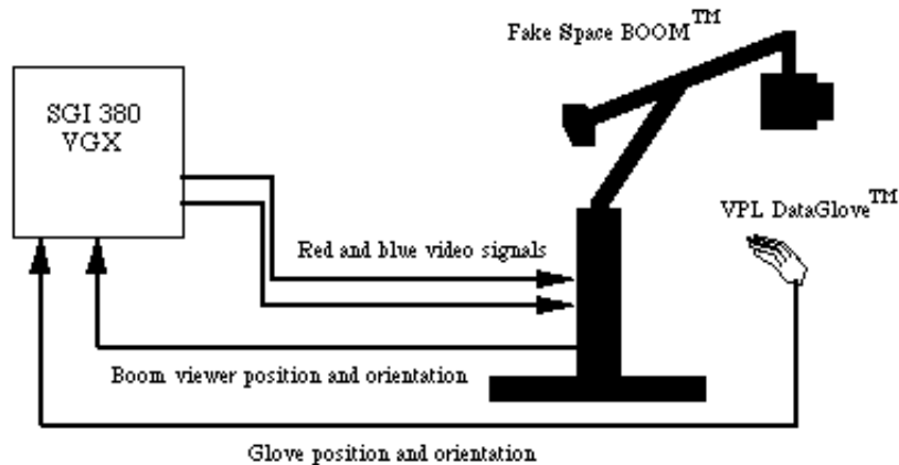
Fig 3: The hardware configuration of the virtual windtunnel system.
