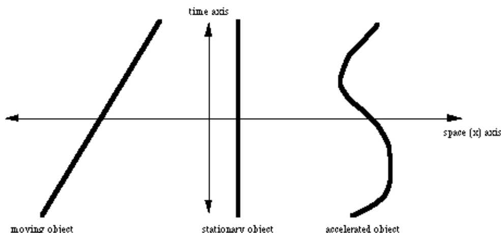
Figure 2. Example spacetime diagram showing world lines in a flat spacetime.
