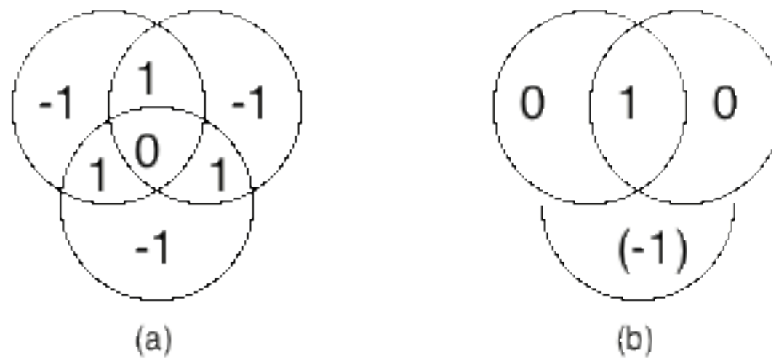
Figure 3: Entropy diagrams for a system of three mutually entangled particles (a) and the same diagram with one particle ignored or "traced over" (b). The total entropy in both cases is 0, but the apparent total entropy in the second case is 1.
