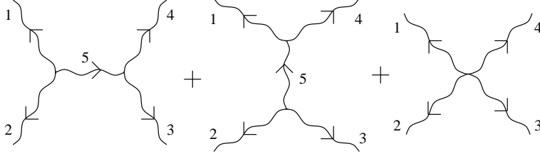
Figure 81.1: The diagrams contributing to the partial amplitude A(1, 2, 3, 4) .
