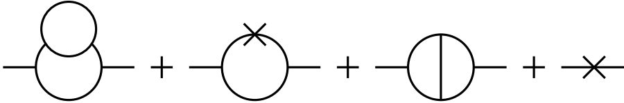
Figure 14.3: The O(g^4) contributions to \Pi(k^2) .
