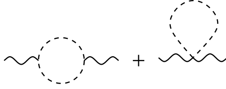
Figure 78.1: The one-loop contributions to the \bar{A} propagator in background field gauge; the dashed lines can be either ghosts or internal \mathcal{A} gauge fields.
