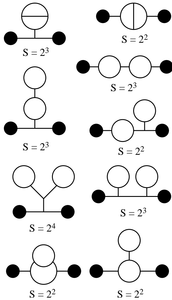
Figure 9.7: Diagrams with E = 2 and V = 4 .
