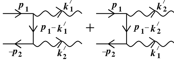
Figure 59.1: Diagrams for e^+e^- \rightarrow \gamma\gamma , corresponding to eq. (59.1).
