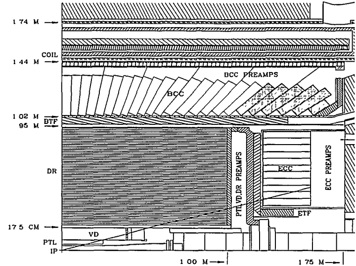
Figure 1: Quarter section of the CLEO II detector.
