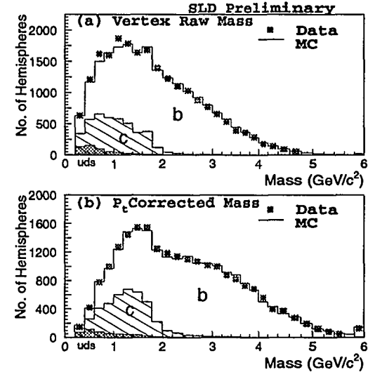
Figure 10: Distributions of (a) raw mass and (b) p_T -added mass for topological vertices.
