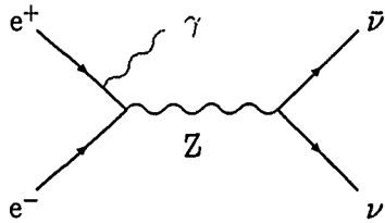
Figure 38: Feynman diagram contributing to the single photon reaction in the SM.
