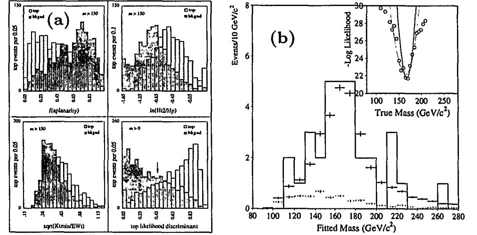
Figure 9: D\bar{D} top mass measurement: (a) Distribution of MC top (light) and background (dark) lepton plus four-jet events for different kinematic parameters like aplanarity, H'_{T2} , K'_{T,\text{min}} , and the combined top likelihood discriminant \mathcal{D} (from top left to bottom right). (b) Observed (solid) top quark mass distribution, where the solid crosses represent the prediction for background plus signal. The dashed crosses are just the background expectation. The curves in the insert are used to determine the top quark mass and its statistical error.
