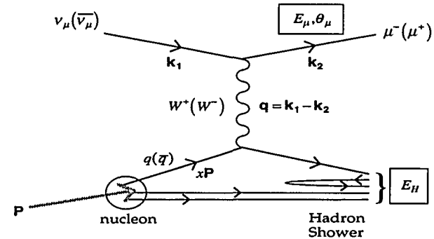
Figure 1: The first-order Feynman diagram for deep inelastic neutrino scattering.
