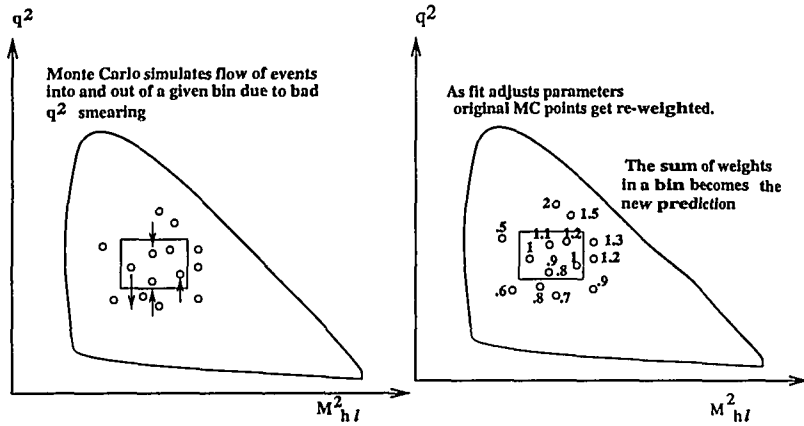
Figure 29: A Monte Carlo simulation using an initial guess for the relevant form factors is used to simulate the q^2 smearing due to neutrino reconstruction. This smearing will cause events to diffuse into and out of each bin. The program saves the generated Dalitz variables as well as the smeared Dalitz variables for each simulated event. As the fitter changes the form factors to minimize w , each simulated event is assigned a weight given by the ratio of the intensity with the new form factors divided by the ratio of the original intensity with the initial guess. The expected number of observed counts \mu_i within a bin is computed from the sum of the weights for events falling within the i 'th bin. This technique avoids prohibitively computer intensive, separate full Monte Carlo simulations for each iteration of the fit.
