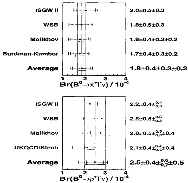
Figure 18: The results for the branching ratios for several models. The central vertical line is the average of the models.
