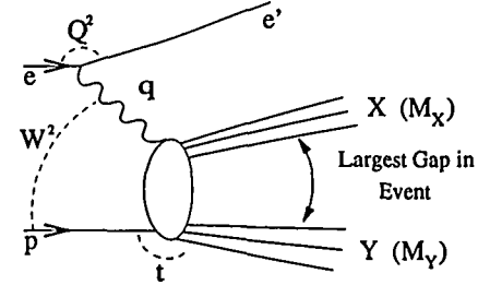
Figure 20: Schematic illustration of the selection method used to define a diffractive cross section by the H1 Collaboration.
