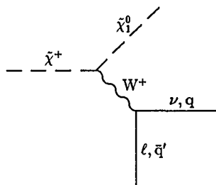
Figure 26: Chargino decay into the lightest neutralino and a W boson.
