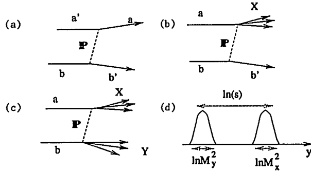
Figure 2: Diagrams for three different types of diffractive reactions: elastic scattering (a), single diffraction (b) where one of the incoming particle fragments, and double diffraction (c). (d) shows energy flow as a function of rapidity for \ln(s) \gg \ln(M_y^2) + \ln(M_X^2) .
