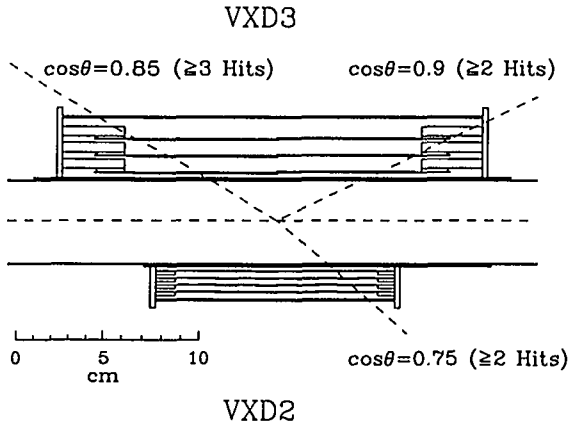
Figure 26: Sideviews of the old (VXD2) and new (VXD3) vertex detectors.
