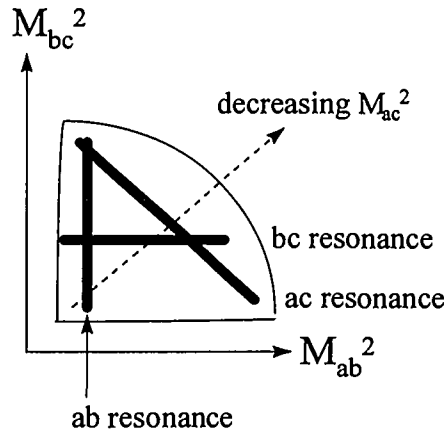
Figure 8. Schematic diagram of a Dalitz plot.
