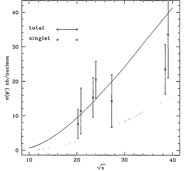
Figure 8: Total (solid) and singlet only (dotted) \psi' production cross section ( x_F > 0 ) in proton-nucleon collisions. The solid line is obtained with M_7^{\psi'}({}^1S_0^{(8)}, {}^3P_0^{(8)}) = 5.2 \cdot 10^{-3} \text{ GeV}^3 .
