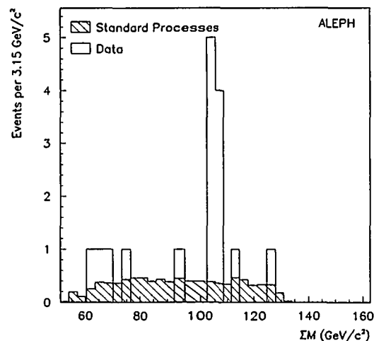
Figure 36: Sum of jet-pair masses in four-jet hadronic events as observed by ALEPH for cms energies of 130-140 GeV.
