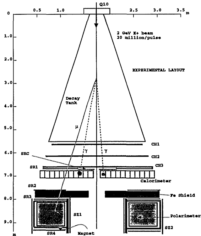
Fig. 12. Proposed apparatus of AGS E923.
