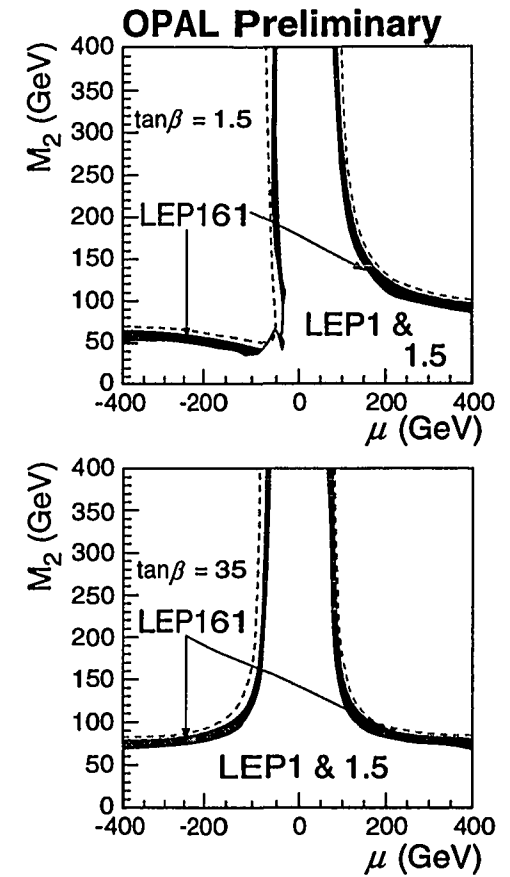
Figure 35: Exclusion (95% C.L.) of SUSY parameters \mu and M_2 for two different values of \tan \beta and for m_0 = 1 TeV from OPAL. The limits obtained from 161 GeV are compared to the combined limits from LEP I and LEP 1.5. The broken lines indicate the kinematic limit at 161 GeV for chargino pair production.
