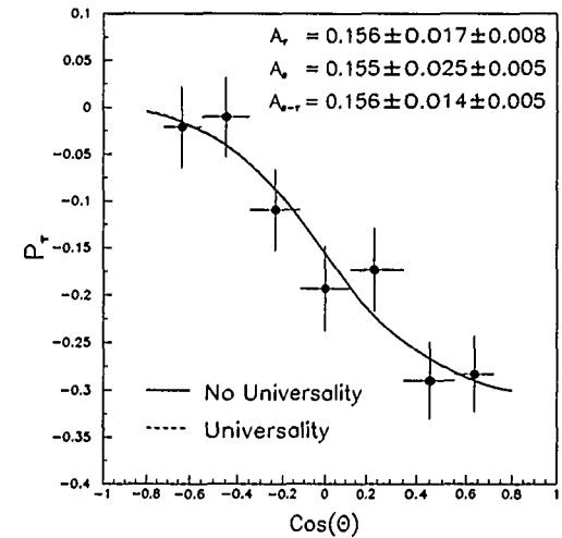
Fig. 5. \tau polarization as a function of the scattering angle from the L3 Collaboration. The line represents a fit to the data with (dashed) and without (solid) the assumption of lepton universality.
