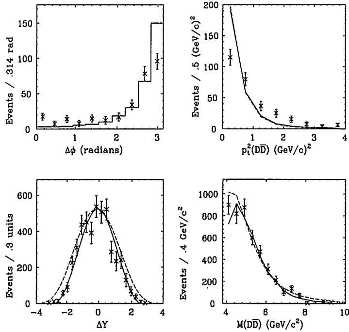
Fig. 12. D\bar{D} kinematic correlations observed in E687 data overplotted with the predictions of the default PYTHIA model. We use the fully reconstructed D\bar{D} sample for the upper row of transverse correlations, and (because of its larger kinematic acceptance domain) the partially reconstructed sample for the lower row which involves longitudinal correlations. The solid curves show acceptance-corrected predictions; the dashed curves show the predictions without acceptance effects.
