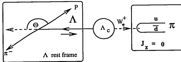
Fig. 61. For \Lambda_c^+ \rightarrow \Lambda \pi^+ , q^2 = m_\pi^2 \rightarrow 0 , HQET predicts \alpha_{\Lambda_c} = -1 .
