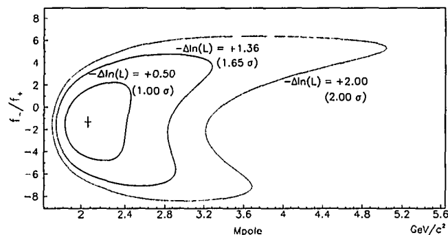
Fig. 38. Contours of constant likelihood for f_-/f_+ versus m_{\text{pole}} assuming that f_- and f_+ follow pole forms with the same pole mass. Note that the contour shape shows that a large f_-/f_+ ratio can be compensated by an increased value for m_{\text{pole}} which can be understood from Eq. (20) for the case where |f_-(q^2)|^2 > 2 f_-(q^2) f_+(q^2) .
