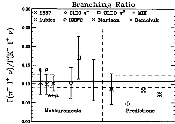
Fig. 48. An informal weighted average gives \Gamma(\pi^- \ell^+ \nu)/\Gamma(K^- \ell^+ \nu) = 0.11 \pm 0.02 . The data slightly exceeds the predictions.
