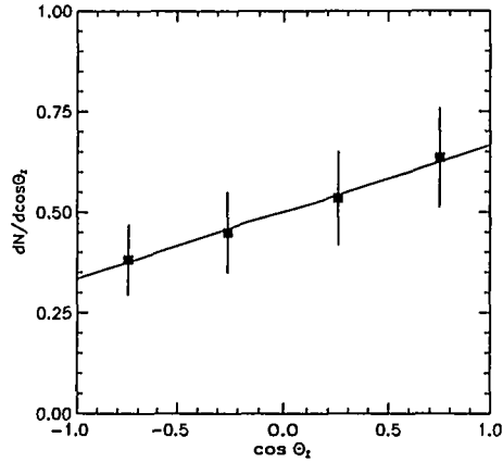
Fig. 63. CLEO's acceptance-corrected measurement of the \Lambda polar angle distribution in the \Xi^- rest frame with respect to the \Xi^- helicity axis in \Xi_c^- \rightarrow \Xi^- \pi^+ decays. The slope of this line divided by the \Xi^- analysis power of -0.46 gives \alpha_{\Xi_c^-} \approx -1 .
