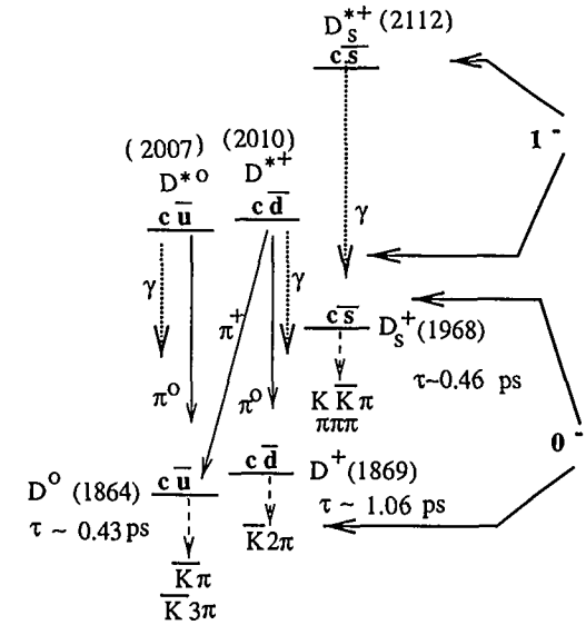
Fig. 1. Sketch of the spectrum of low lying charm mesons. The D^0 and D^+ mesons form a nearly degenerate strong isodoublet. The D_s^+ is shifted upwards by roughly 100 MeV. This mass splitting pattern is repeated for the D^* 's. Weak decays are shown by dashed arrows. Some strong and electromagnetic de-excitations of the D^* system into the ground state D system are shown by solid and dashed arrows. The approximate lifetimes of the ground state D system are indicated on the figure.
