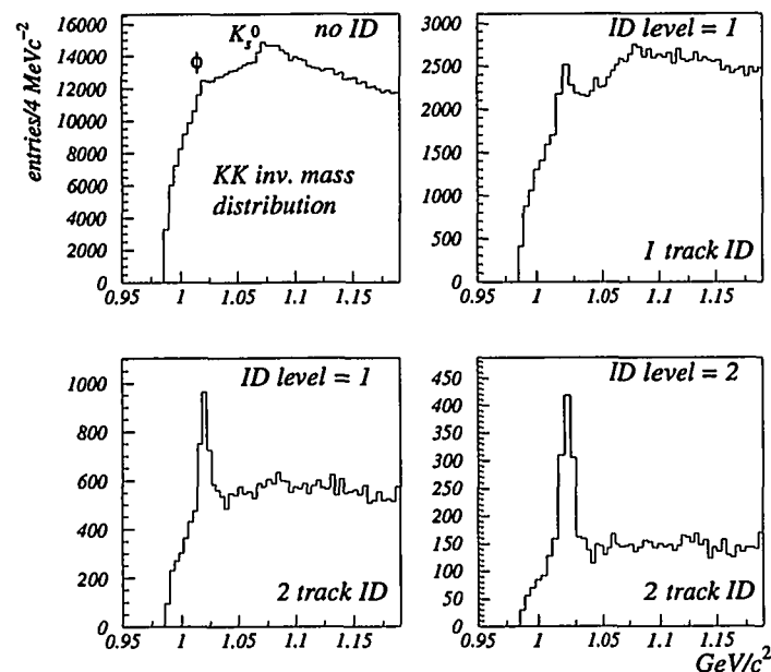
Figure 21: Invariant mass distributions for \phi \rightarrow K^+K^- decay candidates without and with various levels of kaon identification.
