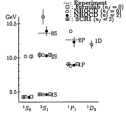
Figure 25: \Upsilon spectrum.
