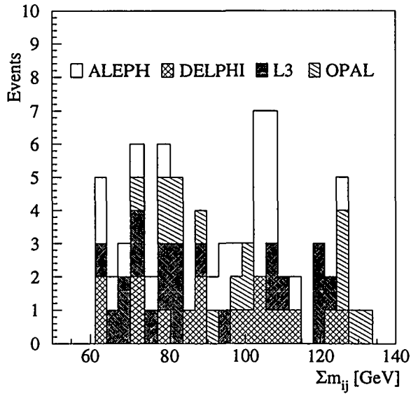
Figure 37: Distribution of the sum of jet-pair masses in four-jet hadronic events as observed by the four LEP experiments at cms energies of 130–140 GeV.
