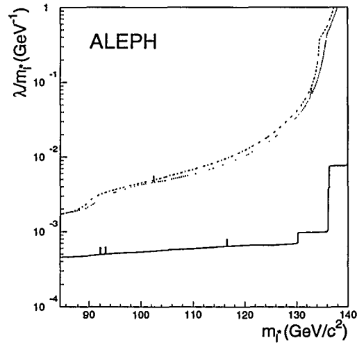
Figure 41: Exclusion limits (95% C.L.) in the mass-coupling plane for singly produced charged leptons \ell^* as obtained by ALEPH at LEP 1.5. The solid, dotted, and dot-dashed lines are for e^* , \mu^* , and \tau^* , respectively. 44
