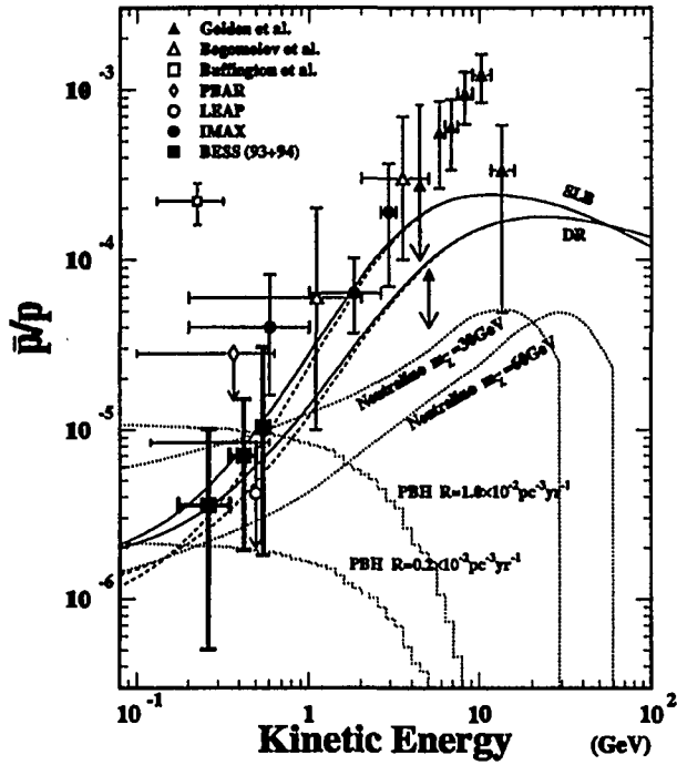
Figure 11: Measured \bar{p}/p ratio in comparison with the other experimental data and calculations. Filled squares, the present result; filled triangles, Golden et al. ; open triangles, Bogomolov et al. ; open square, Buffington et al. ; open diamond, the PBAR experiment; open circle, the LEAP experiment; filled circles, the recent result of IMAX. The dashed curves labeled “SLB” and “DR” are recently calculated by Mitsui based on the Standard Leaky Box Model and Diffusive Re-acceleration Model, respectively. The dotted curves labeled “PBH” are predictions of Maki et al. for the \bar{p} ’s produced by primordial black holes with two different assumed evaporation rates R . The dotted lines labeled “Neutralino” are the prediction of Jungman and Kamionkowski for the \bar{p} productions by annihilations of dark matter neutralinos.
