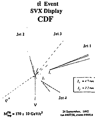
Figure 5: Example of a SVX-tagged event where both b jets are SVX tagged.
