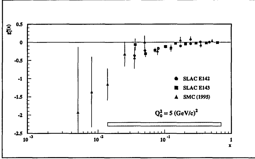
Fig. 3. Published data for g_1^n(x) . The shaded region indicates the x interval of the present experiment.
