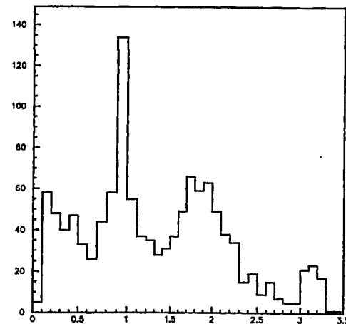
Figure 38. Mass \pi^+\pi^- squared from experiment E791.
