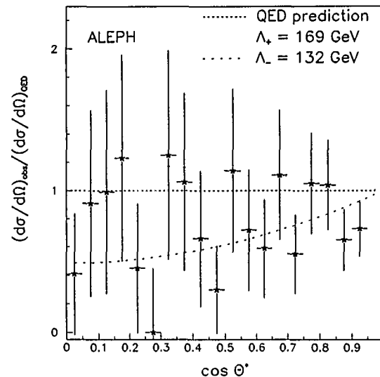
Figure 40: Ratio of the experimental and QED expected differential cross section of the reaction e^+e^- \rightarrow \gamma\gamma as measured by ALEPH at cms energies between 130 and 140 GeV (Ref. 40). The two lines show the maximum deviation experimentally allowed according to the parameterization of Eq. (15) from which limits for \Lambda_{\pm} are derived.
