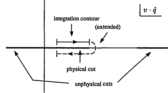
Figure 4: Analytic structure of T^{\mu\nu} in the complex v \cdot \hat{q} plane, for fixed, real \hat{q}^2 . The integration contour is over the “physical cut,” corresponding to real decay into leptons. The unphysical cuts correspond to other processes.
