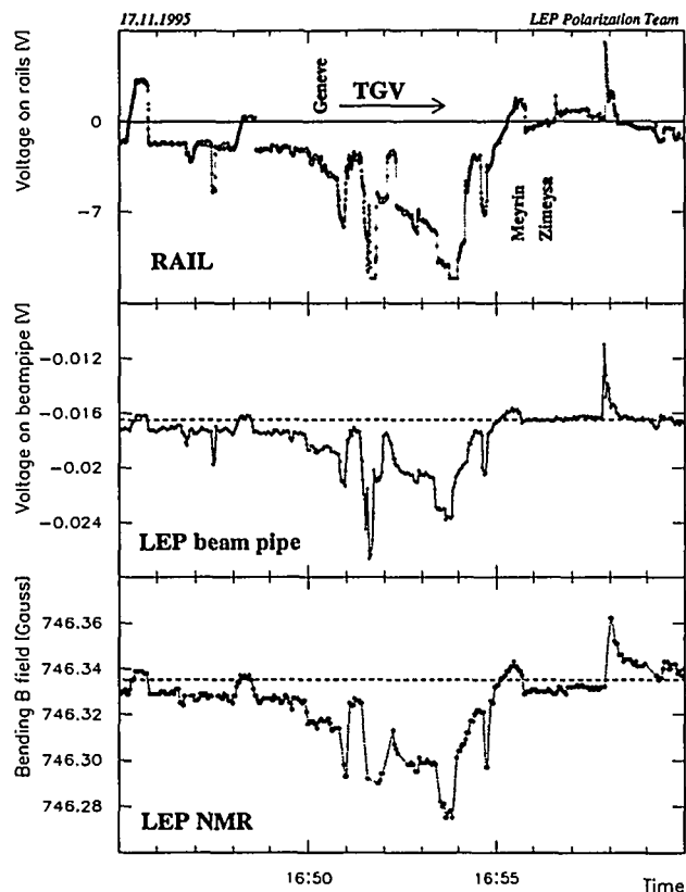
Fig. 1. Effect of trains on the LEP beam energy. The upper plot shows the voltage measured on the rails while a train is passing close to the LEP tunnel. The middle plot shows the voltage measured simultaneously on the LEP beam pipe, and the lower plot shows the field of the dipole magnets measured by an NMR probe.
