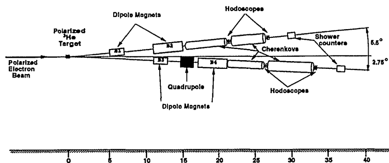
Fig. 7. Schematic of the 2.75° and 5.5° spectrometers as seen from above.
