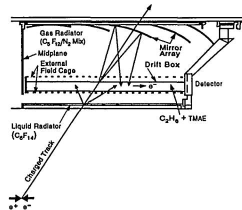
Figure 3: Cross-section view of one CRID quadrant.
