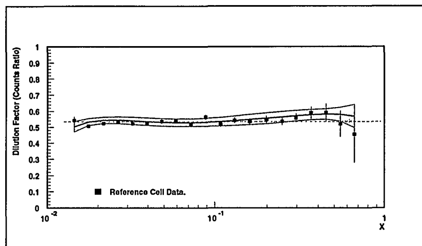
Fig. 6. Dilution factor as determined by mechanical measurement and as determined by reference cell rate measurement (symbols). The band is the result of the calculation based on the parameterization of the cell.
