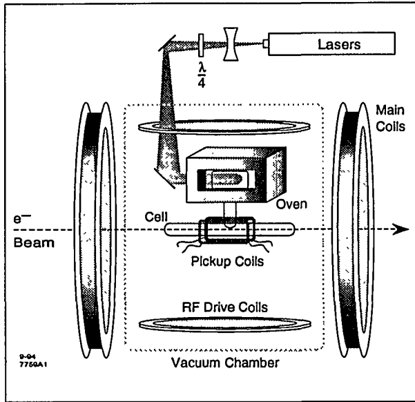
Fig. 4. Schematic of laser-polarized ^3\text{He} target.
