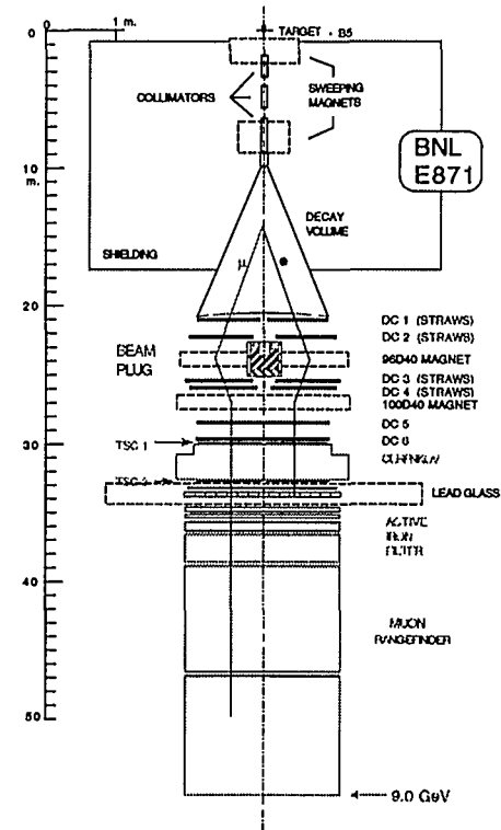
Fig. 3. Apparatus of AGS E871.
