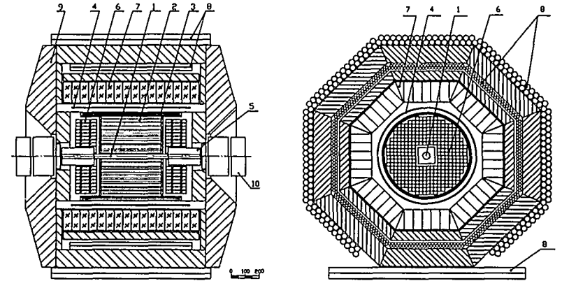
Figure 2: Horizontal and vertical cross sections of the CMD-2 detector. (1) Vacuum chamber; (2) drift chamber; (3) Z chamber; (4) main solenoid; (5) compensating solenoid; (6) BGO end cap calorimeter; (7) CsI barrel calorimeter; (8) muon range system; (9) magnet yoke; (10) collider lenses.
