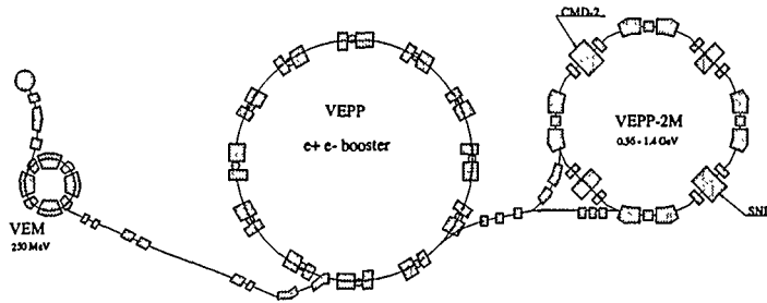
VEPP-2M Layout
