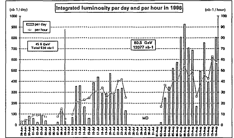
Figure 1: Day-by-day development of the integrated luminosity per day and per hour delivered by LEP to each experiment from the end of June to August 1996.
