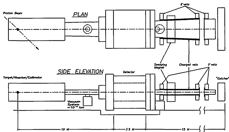
Fig. 11. Proposed apparatus of AGS E926.
