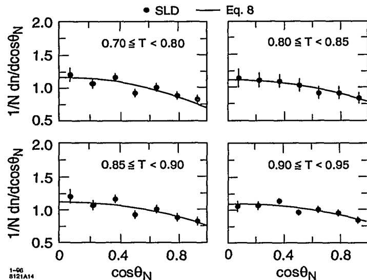
Figure 12: Distributions of \cos\theta_N as a function of event thrust from SLD [21].
