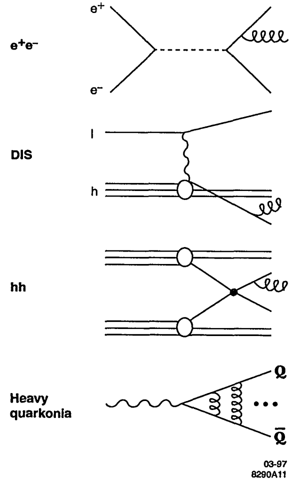
Figure 1: Schematic of the production of hadronic final states by different interactions: e^+e^- annihilation, deep inelastic lepton-hadron scattering, hadron-hadron collisions, and production and decay of heavy quarkonia.
