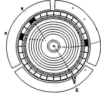
Fig. 1. Typical CPLEAR event.
