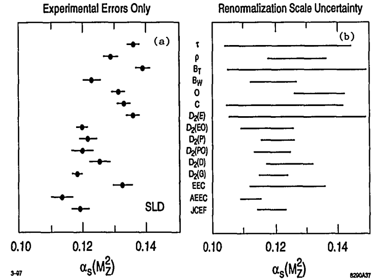
Figure 34: (a) Values of \alpha_s(M_Z^2) determined [57] by fitting O(\alpha_s^2) QCD predictions to 15 hadronic event shape observables using a fixed value of the renormalization scale \mu = Q ; the results are clearly inconsistent within the experimental errors. (b) Renormalization scale uncertainties.
