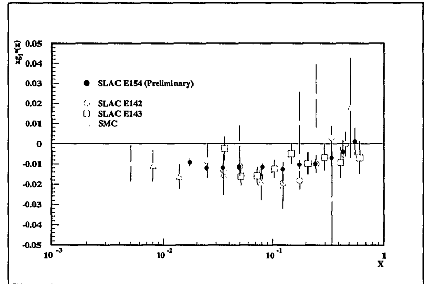
Fig. 10. Comparison of results of E154 and the rest of the world for the spin structure function g_1^n(x) evolved to a common Q^2 of 5 (GeV/c) 2 . Evolution is done with Eq. (26).
