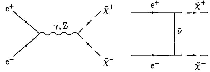
Figure 24: Feynman diagrams contributing to SUSY chargino pair production.
