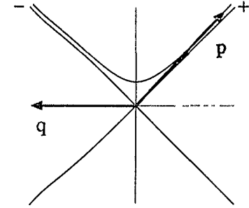
Figure 21: Reference frame for the analysis of deeply inelastic scattering.
