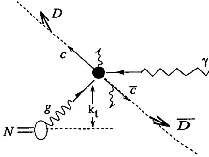
Figure 5: A cartoon of photoproduction of charm in the real world which illustrates several nonperturbative effects. The incident gluon can be thought to carry a small momentum component transverse to the incident nucleon called k_t . Soft gluon emission can accompany the charmed quark as it dresses, creating additional sources of relative P_\perp . A significant amount of quark energy is lost to the emerging D 's while they hadronize.
