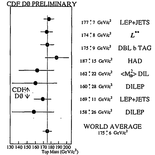
Figure 10: Summary of the CDF and DØ top quark mass measurements in different decay channels.
