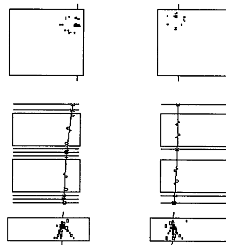
Figure 8: Display of a single 2.2 GeV/c antiproton traversing the CAPRICE apparatus. The antiproton interacts in the calorimeter showing clearly several charged particles emerging from the vertex of interaction; this could be an annihilation in flight.
