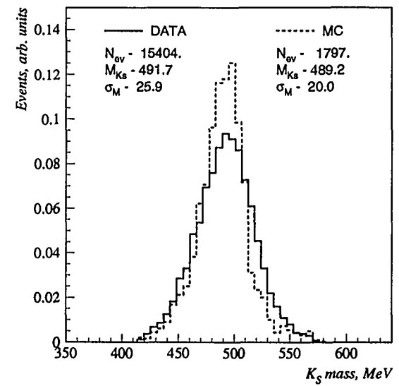
Figure 19: Effective mass spectrum of four photons from K_S \rightarrow 2\pi^0 decay.
