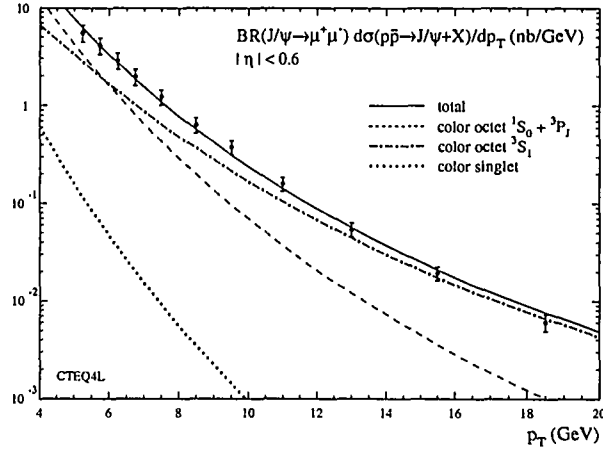
Figure 5: Fit of color octet contributions to direct J/\psi production data from CDF ( \sqrt{s} = 1.8 TeV, pseudorapidity cut |\eta| < 0.6 ). Theory: CTEQ4L parton distribution functions, the corresponding \Lambda_4 = 235 MeV, factorization scale \mu = (p_t^2 + 4m_c^2)^{1/2} , and m_c = 1.5 GeV. Taken from Ref. 37.
