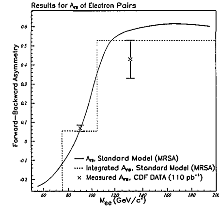
Figure 6: Z charge asymmetry (CDF preliminary).
