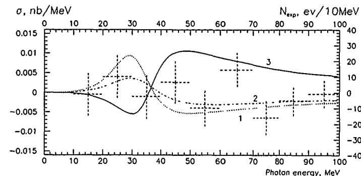
Figure 7: Difference in spectrum for gammas in the “ \phi ” and “non- \phi ” regions, normalized to integrated luminosity. The solid lines represent the theoretical prediction for the four-quark model of the 2.4 \times 10^{-4} branching ratio in the case of (1) positive and (3) negative interference signals with a 40 MeV f_0 width. Line (2) is a negative interference signal with a 100 MeV f_0 width.
