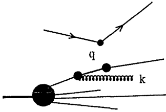
Figure 27: Deeply inelastic scattering with a gluon emission.
