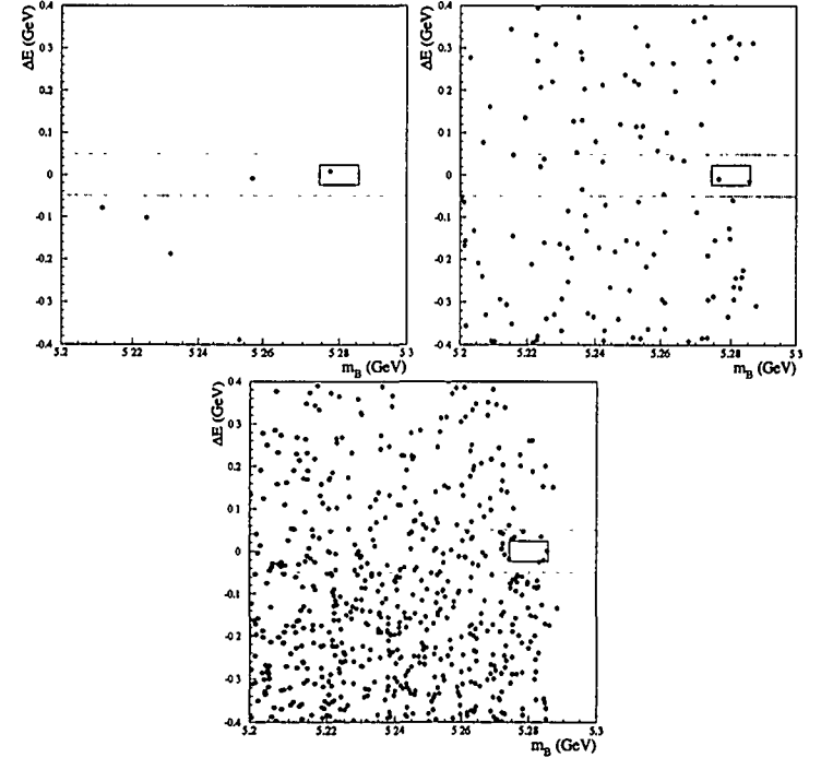
Figure 2: \Delta E vs m_B for data. The signal region is indicated by the box. The sideband region lies above and below the dotted lines.
