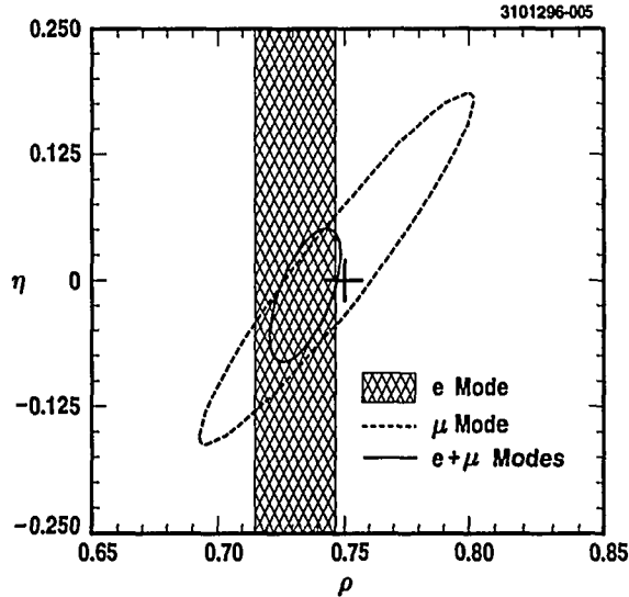
Figure 23: \rho vs \eta for electron, muon, and combined modes. The Standard Model prediction is given by the cross.
