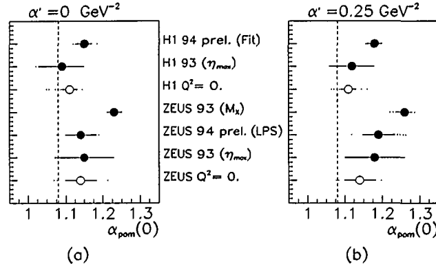
Figure 27: Compilation of \alpha_p(0) values obtained at HERA, assuming, for the measurement at large Q^2 , (a) \alpha'_p = 0.0 \text{ GeV}^{-2} ; or (b) \alpha'_p = 0.25 \text{ GeV}^{-2} . Empty dots are values obtained at Q^2 = 0 \text{ GeV}^2 , full dots at high Q^2 . The dashed vertical line is the value \alpha_p(0) = 1.08 . The solid line is the statistical error while the dotted line is the systematic error.
