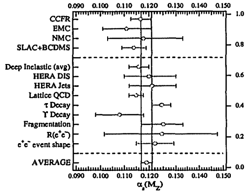
Figure 15: Measurement of \alpha_s from various experiments. The CCFR result is preliminary. Results from other experiments are from Ref. 23.
