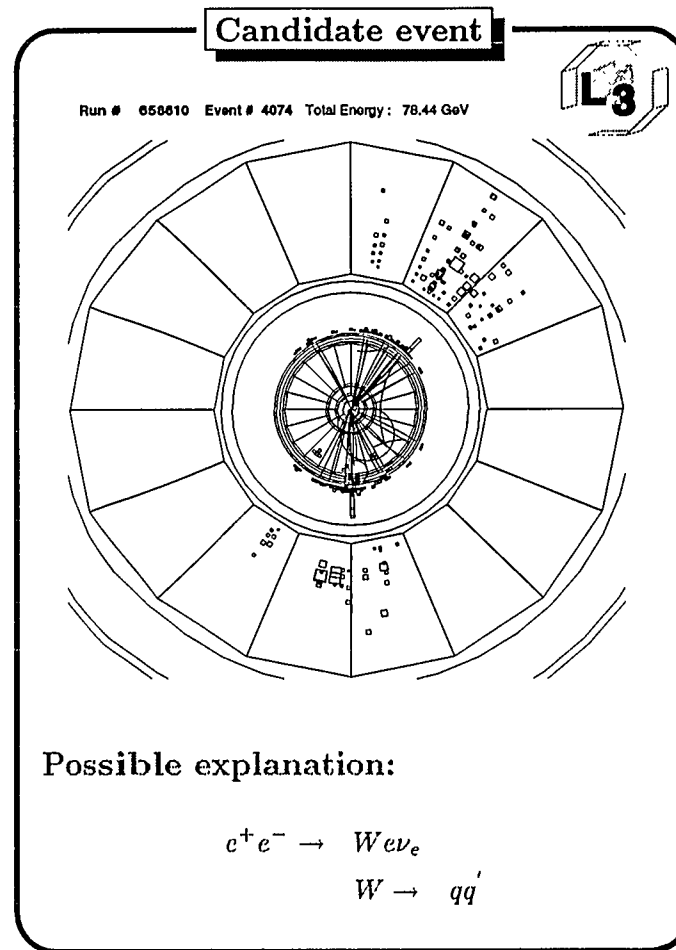
Figure 28: Two-jet hadronic event with missing energy observed by L3 at \sqrt{s} = 161 GeV. The SM explanation for this event is single W production with the electron escaping detection through the beam pipe (Fig. 27).
