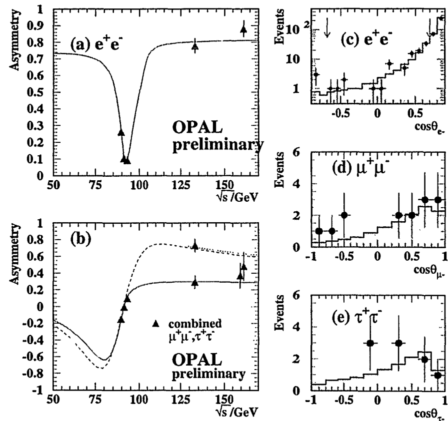
Figure 9: Measured e^+e^- forward-backward asymmetry (a) for |\cos\theta_{e^-}| < 0.7 as a function of the cms energy as obtained by OPAL. (b) shows the combined muon and tau asymmetry as a function of energy for the total and the high-energy samples ( \sqrt{s'}/s > 0.8 ). The SM expectations are represented as solid lines for the total, and a dotted line for the high-energy sample. The broken line shows the Born-level asymmetry. The polar angle distributions at 161 GeV of the negative leptons are shown in plots (c)-(e).
