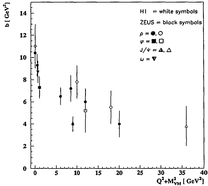
Figure 16: Exponential slope b for vector meson production as a function of Q^2 + M_{VM}^2 .
