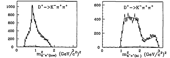
Fig. 76. Comparison of the lower and higher K^- \pi^+ mass projection in E687 data (error bars) and our fit (histogram). The high projection does not match near 2.5 \text{ GeV}^2 .
