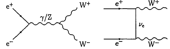
Figure 17: Feynman diagrams contributing to the reaction e^+e^- \rightarrow W^+W^- in lowest order.
