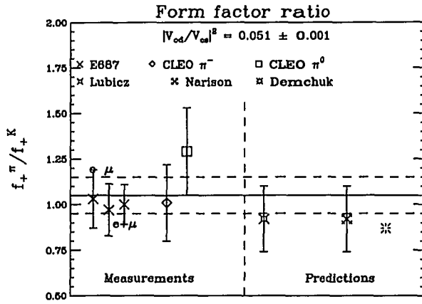
Fig. 49. An informal weighted average of the form-factor ratio is |f_+^\pi/f_+^k| = 1.05 \pm 0.095 (assuming |V_{cd}/V_{cs}|^2 = 0.051 ). The predictions are in reasonably good agreement with the prediction.
