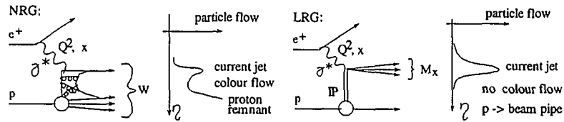
Figure 29. Comparison of ep events with no rapidity gap (NRG) and with a large rapidity gap (LRG), showing the absence of the particle and color flow in LRG events.
