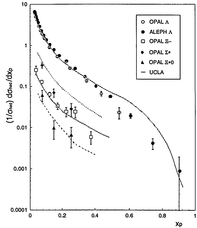
Fig. 18. UCLA predictions for various strange baryons are compared to experiments at E_{CM} = 91 GeV.
