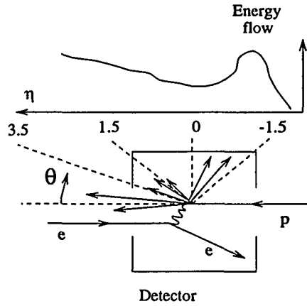
Figure 5: Energy flow vs \eta for nondiffractive ep scattering at HERA.
