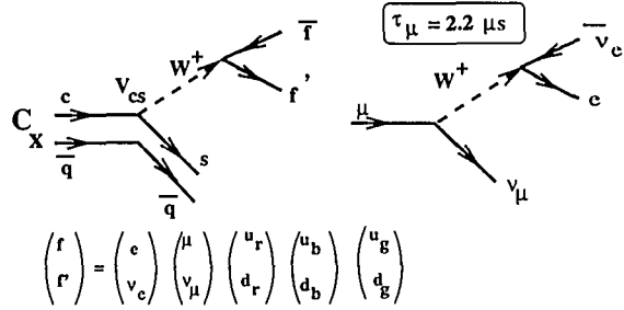
Figure 18: In the naive spectator model, the lifetime of charmed particles should have a universal value which can be estimated by scaling from the known muon lifetime of 2.2 \mu s . When scaling decay rates, one would need to consider the fact that five low mass final states are available for the charmed quark (two lepton generations and three color multiplets of the first quark generation), and that the charm quark has a much larger decay phase space owing to its much larger mass.
