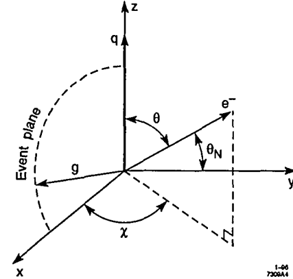
Figure 11: Definition of event-plane orientation angles.
