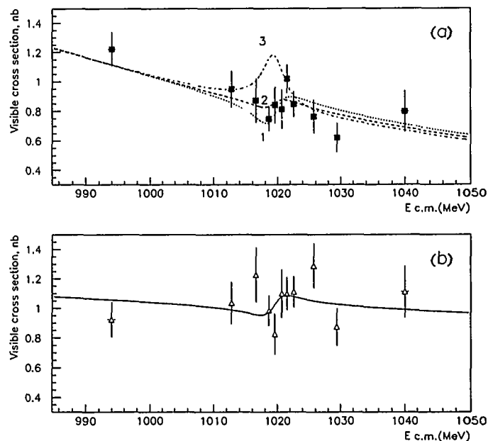
Figure 6: (a) Visible cross section for e^+e^- \rightarrow \pi^+\pi^-\gamma . Lines are theoretical predictions for the case of no f_0\gamma signal (2), an f_0\gamma signal with B(\phi \rightarrow f_0\gamma) = 2.4 \times 10^{-4} for a negative relative phase (3), and a positive relative phase (1). (b) Visible cross section for e^+e^- \rightarrow \mu^+\mu^-\gamma , compared with theoretical prediction.
