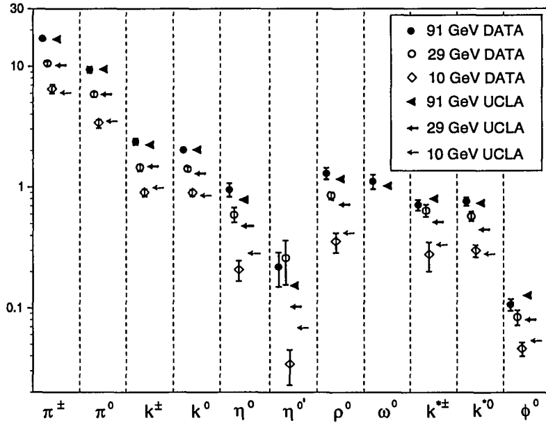
Fig. 9. Comparison of the experimental and predicted absolute production rates per event for various flavored light-quark mesons at E_{CM} = 10, 29 , and 91 GeV.
