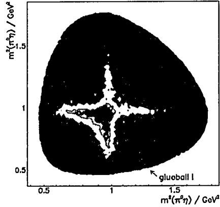
Figure 15. Dalitz plot for p\bar{p} \rightarrow \eta\eta\pi^0 from the Crystal Barrel.
