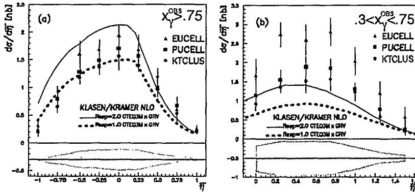
Figure 25. Differential dijet cross section, d\sigma/d\eta \ln|b| , for three different jet algorithms from ZEUS for (a) direct photoproduction and (b) resolved photoproduction. The shaded band indicates the uncertainty due to the \pm 5\% uncertainty in the calorimeter energy scale. The curves are from the full QCD NLO calculations described in the text.
