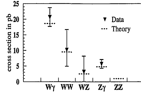
Diboson cross sections from CDF (preliminary)
