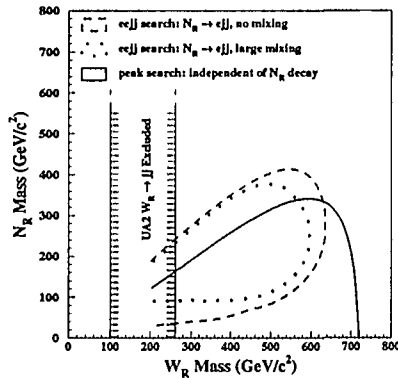
Figure 16: DØ right-handed W search.
