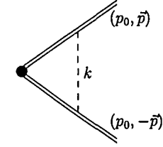
Figure 1: Coulomb correction to point-like \psi^\dagger \chi creation.
