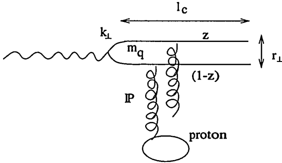
Figure 8: Diffractive \gamma p scattering in the proton rest frame.
