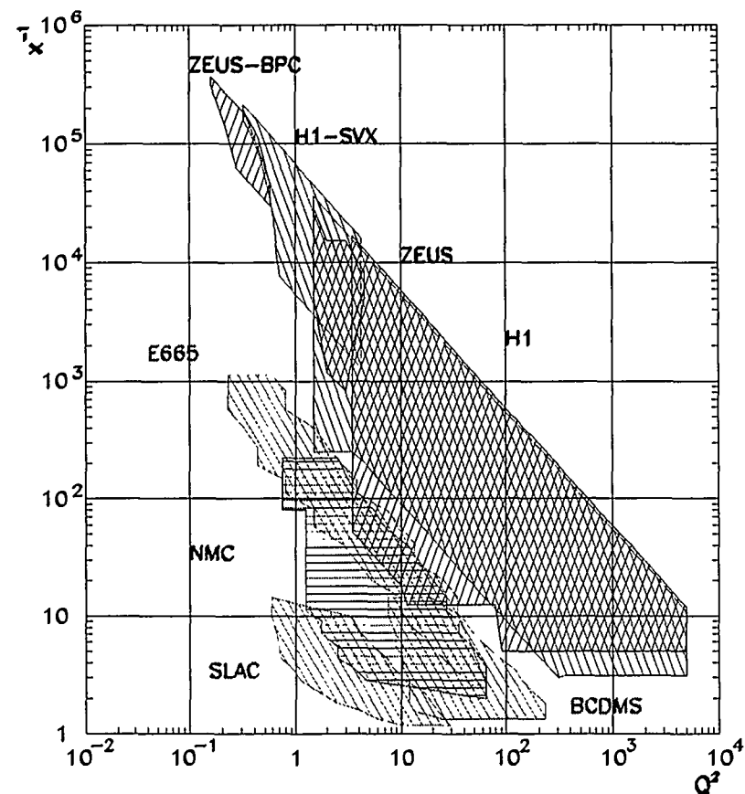
Figure 6. Kinematic range of structure function measurements.
