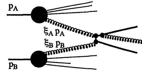
Figure 35: Feynman graph for heavy quark production. The lowest order hard process is g + g \rightarrow Q + \bar{Q} , which occurs at order \alpha_s^2 . This particular Feynman diagram illustrates an order \alpha_s^3 process in which a gluon is emitted.
