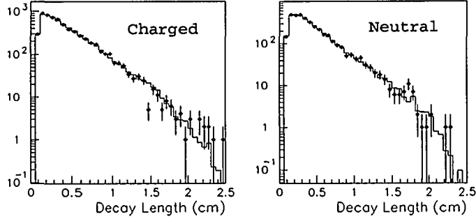
Figure 13: Decay length distributions for data (points) and best fit Monte Carlo (histogram) in the topological analysis.
