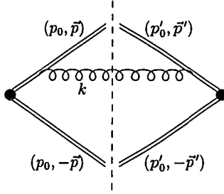
Figure 3: Contribution to mixing of \langle \mathcal{O}_8^\psi(^3S_1) \rangle into \langle \mathcal{O}_1^\psi(^3P_0) \rangle .
