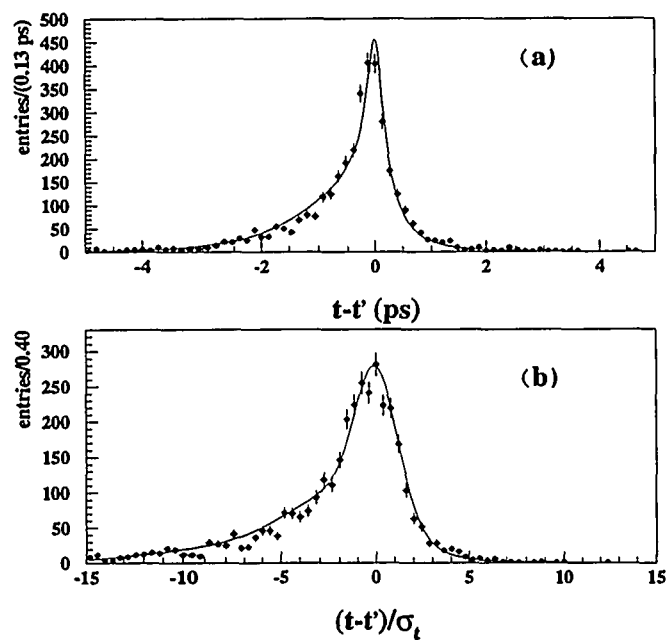
Fig. 18. (a) Difference between the reconstructed proper time t and the true proper time t' in the OPAL D^{*\pm}l analysis. The points are the data, and the solid line is the prediction from the Monte Carlo. (b) Same as (a) divided by the calculated error on t .
