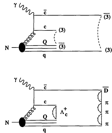
Figure 14: In JETSET, strings are drawn between the triplet and anti-triplet color poles. Final-state hadrons are produced as these strings fragment. Quarks are color triplets; antiquarks are color anti-triplets. In photon-gluon fusion, the initially colorless nucleon emits a color octet gluon. The nucleon remnants must therefore form a color octet to "cancel" the color of the gluon. JETSET achieves color conservation by resolving the nucleon remnants into an anti-triplet, effective di-quark ( Q ), and a triplet, effective quark ( q ). Because the c quark must dress with the q remnant and the \bar{c} quark must dress with the Q remnant, a difference between the quark and di-quark momenta fraction distributions will lead to an asymmetry between the momenta spectra of the charmed and anti-charmed hadrons.
