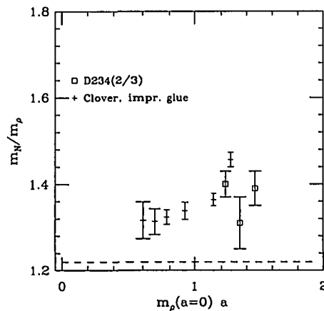
Figure 19: Nucleon to rho mass ratio (at chiral limit) vs lattice spacing (in units of 1/m_\rho ).
