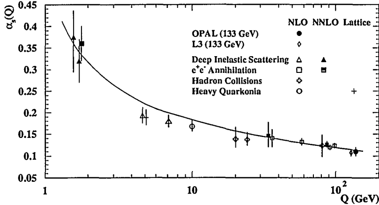
Figure 16: Measurement of the strong coupling constant \alpha_s at different energies. New LEP measurements at \sqrt{s} = 133 \text{ GeV} are compared to measurements at the Z and various other determinations at lower energies. The solid line represents the second order QCD prediction for \alpha_s(m_Z) = 0.120 (Ref. 20).
