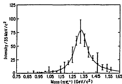
Fitting of the Breit-Wigner formula to the D_+ wave.
