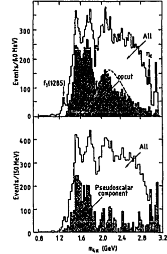
Figure 19. J/\psi \rightarrow \gamma 4\pi from the DM2 group. 23
