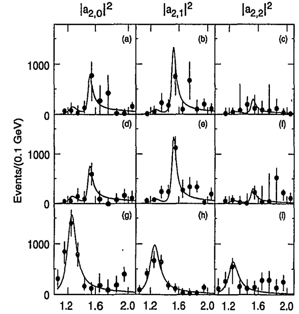
Figure 33. Tensor intensities for helicities 0,1,2 for (a)–(c) K_s K_s , (d)–(f) K^* K^- , and (g)–(i) \pi^+ \pi^- from Mark III.
