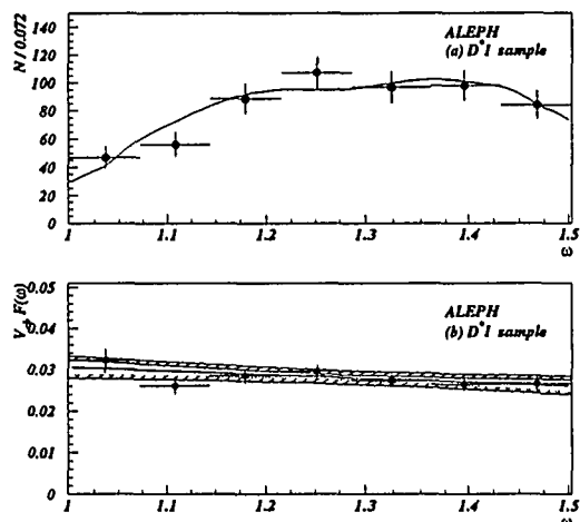
Fig. 16. (a) Differential event rate dN/d\omega after cuts and background subtraction. The points are the data and the solid line is the result of the fit. (b) \mathcal{F}(\omega)|V_{cb}| as a function of \omega . The points are the data, corrected for all detector effects and kinematic terms. The solid line is the result of the fit. The shaded area represents its statistical error and the hatched line its systematic uncertainty.
