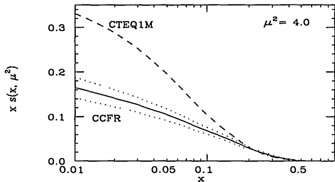
Figure 14: Solid—the strange sea as measured by the CCFR Collaboration from the dimuon data. The surrounding dots show the statistical and systematic errors combined. Dashed—the strange sea required to account for the neutrino-charged-lepton discrepancy, as determined by Ref. 19.
