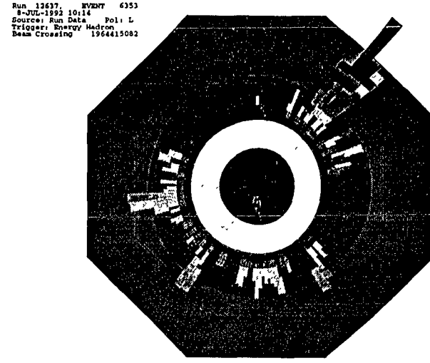
Figure 7: A contemporary three-jet event recorded by SLD: the process e^+e^- \rightarrow Z^0 \rightarrow q\bar{q}g .
