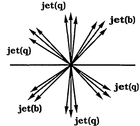
Figure 4: Top decay signature of the all hadronic channel.
