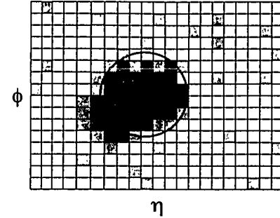
Figure 37: Jet definition according to the Snowmass algorithm. The shading of the squares represents the density of transverse energy as a function of azimuthal angle \phi and pseudorapidity \eta . The cells inside the circle constitute the jet.
