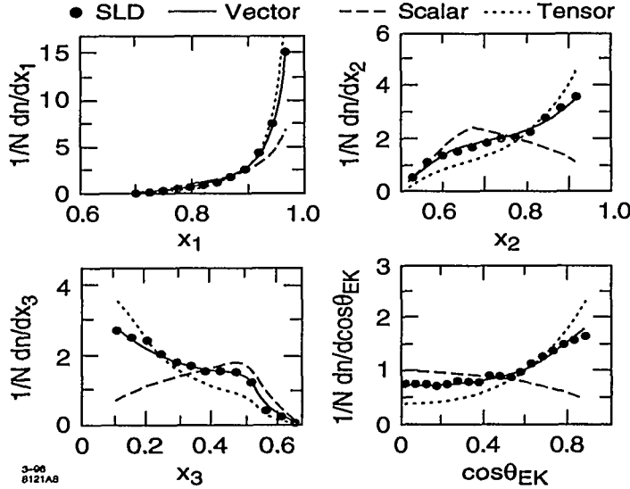
Figure 10: Comparison of leading-order scalar-, vector-, and tensor-gluon models with SLD data [21]; the scalar and tensor hypotheses are clearly excluded.
