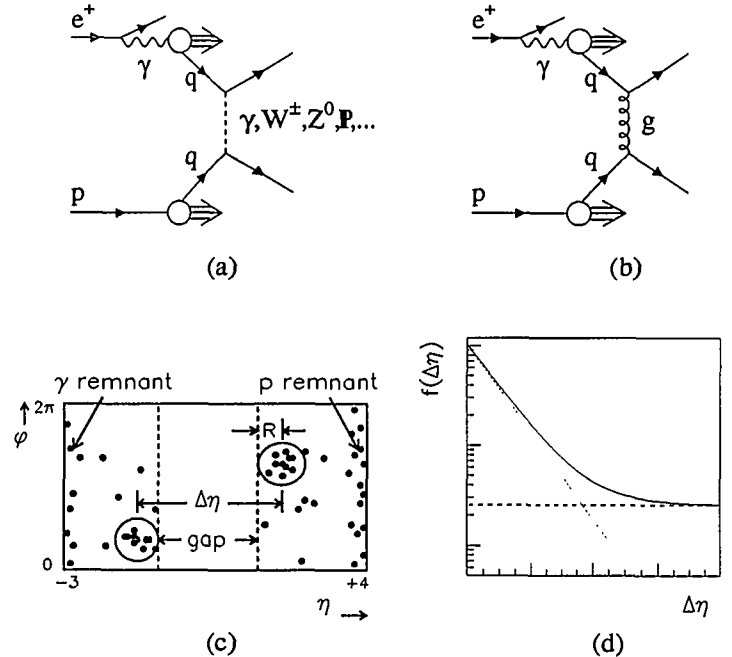
Figure 33: Resolved photoproduction via (a) color singlet exchange and (b) color nonsinglet exchange. The rapidity gap event morphology is shown in (c), where black dots represent final state hadrons and the boundary illustrates the limit of the ZEUS acceptance. Two jets of radius R are shown, which are back-to-back in azimuth and separated by a pseudorapidity interval \Delta\eta . An expectation for the behavior of the gap fraction is shown in (d)(solid line). The nonsinglet contribution is shown as the dotted line and the color singlet contribution as the dashed line.
