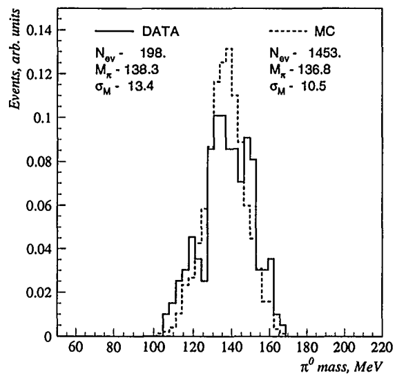
Figure 18: Effective mass spectrum of two photons from the e^+e^- \rightarrow \pi^0\gamma \rightarrow 3\gamma reaction.
