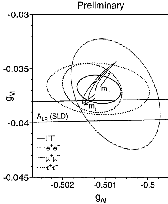
Fig. 7. Contours of 68% probability in the g_{V\ell} - g_{A\ell} plane from LEP measurements. The solid contour results from a fit assuming lepton universality. Also shown is the one standard deviation band resulting from the A_{LR} measurement of SLD. The grid corresponds to the Standard Model prediction for m_t = 175 \pm 6 GeV and m_H = 300^{+700}_{-240} GeV. The arrows point in the direction of increasing values of m_t and m_H .
