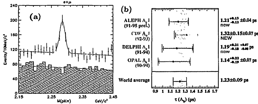
Figure 19: \Lambda_b^0 lifetime measurement: (a) Invariant pK\pi mass distribution for right sign \Lambda_b^0 \ell^- combinations. The shaded histogram shows the wrong sign distribution. (b) Comparison of the CDF \Lambda_b^0 lifetime measurement with LEP results.
