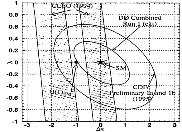
Figure 12: Limits on W anomalous couplings.
