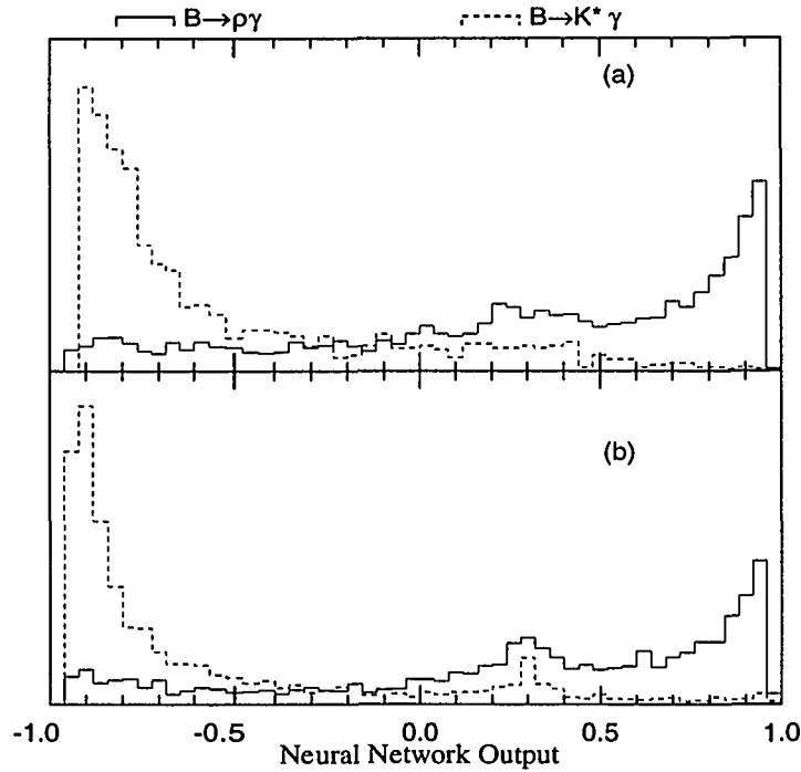
Figure 7: Distribution of the output of the neural network for Monte Carlo samples of (a) B^0 \rightarrow \rho^0 \gamma and B^0 \rightarrow K^{*0} \gamma ( K^{*0} \rightarrow K^+ \pi^- ) and (b) B^- \rightarrow \rho^- \gamma and B^- \rightarrow K^{*-} \gamma ( K^{*-} \rightarrow K^- \pi^0 ).
