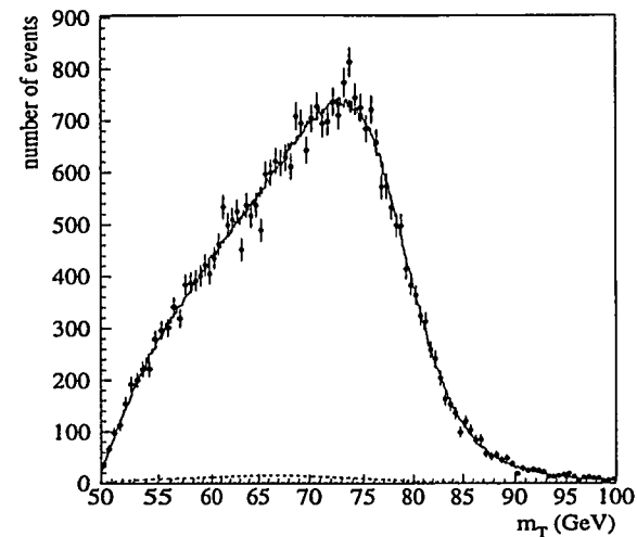
Figure 9: DØ run 1B M_T(e\nu) (preliminary).
