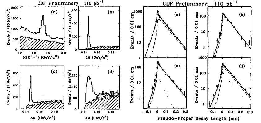
Figure 14: Invariant mass distribution of D^{(*)} candidates (left-hand side) and proper time distributions (right-hand side) from the B -lifetime analysis using partially reconstructed B \rightarrow D^{(*)}\ell X decays with (a) D^0 \rightarrow K^-\pi^+ , where the D^0 is not from a D^{*+} . (b) D^{*+} \rightarrow D^0\pi^+ , D^0 \rightarrow K^-\pi^+ . (c) D^{*+} \rightarrow D^0\pi^+ , D^0 \rightarrow K^-\pi^+\pi^-\pi^- . (d) D^{*+} \rightarrow D^0\pi^+ , D^0 \rightarrow K^-\pi^+\pi^0 .
