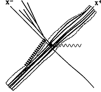
Figure 23: The virtual photon meets the fast moving hadron. One of the partons is annihilated and recreated as a parton with a large minus component of momentum. This parton develops into a jet of particles.
