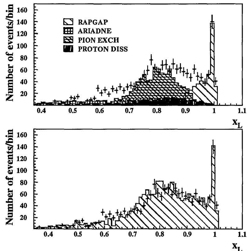
Figure 34. x_L = p'/p_{\text{beam}} distribution for ZEUS data compared with individual (upper plot) and summed (lower plot) MC calculations of events from DIS (ARIADNE), pion exchange, proton dissociation, and diffraction (RAPGAP).
