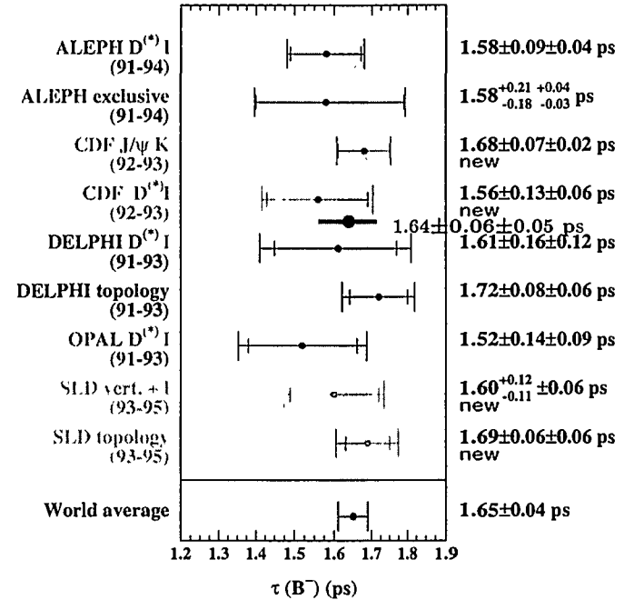
Figure 15: Comparison of the CDF B^+ lifetime measurements with other experiments.
