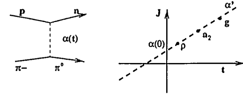
Figure 1: Schematic diagram for \pi^- p \rightarrow \pi^0 n scattering and the exchanged trajectory.
