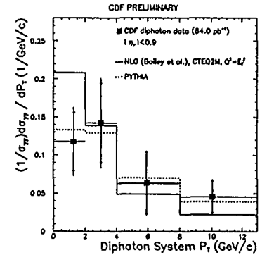
Figure 18: The distribution in p_T of the \gamma\gamma pair. This should be a useful probe of k_T effects.
