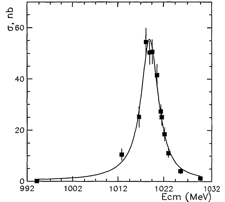
Figure 3: The \phi \rightarrow \eta\gamma cross section.
