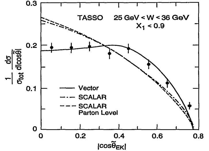
Figure 9: The Ellis-Karliner angle distribution of three-jet events recorded by TASSO at Q \sim 30 GeV (Ref. [18]); the data favor spin-1 (vector) gluons.
