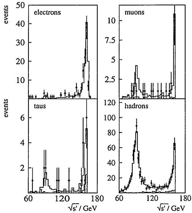
Figure 6: Distributions of the reconstructed effective cms energy \sqrt{s'} for the four reactions of Eq. (1) obtained at \sqrt{s} = 161 GeV by L3. The points with error bars represent the data. Signal and background MC expectations are shown as open and hatched histograms, respectively.
