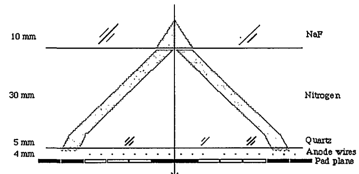
Figure 4: A schematic view of the NaF-RICH detector.
