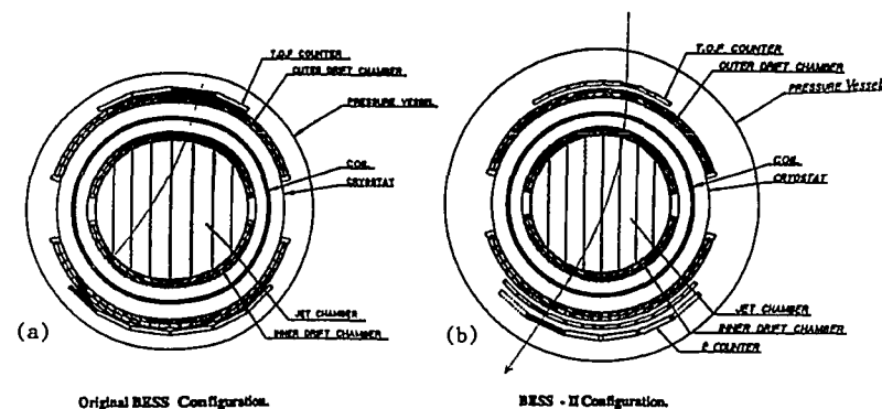
Figure 9: Cross sections of BESS spectrometer.
