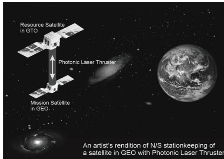
Fig. 9. PLT stationkeeping for north/south orbit maintenance for a GEO spacecraft originally envisioned by Peck. [38]
