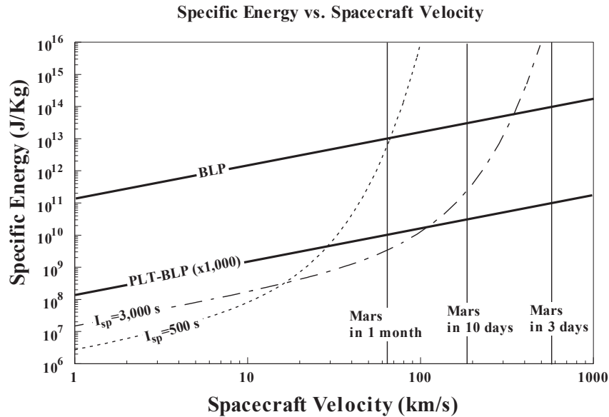
Fig. 11. Specific energy as a function of spacecraft velocity relevant to Mars missions. The flight time to Mars is for flyby missions, and rendezvous missions would take more than twice longer.
