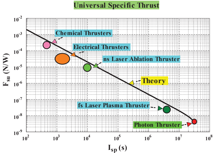
Fig. 1. The overall specific thrust (thrust to power ratio) of representative propulsion systems. Without photon thrust amplification, the specific thrust of photon thrusters follows the classic trend: the higher I_{sp} , the lower the specific thrust. The trend can be explained by the universal specific thrust in Eq. 9. However, with photon thrust amplification by recycling greater than 1,000, the photon thruster can be comparable with other conventional thrusters.
