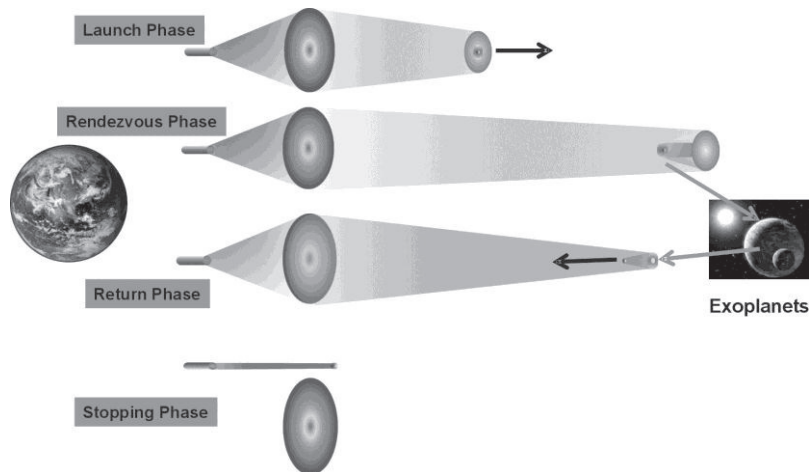
Fig. 2. A four stage roundtrip interstellar flight based on BLP proposed by Forward (1984).
