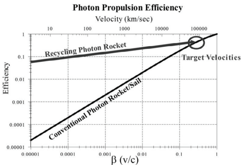
Fig. 4. Energy transfer efficiency from the photon energy to the spacecraft kinetic energy as a function of \beta=v/c .
