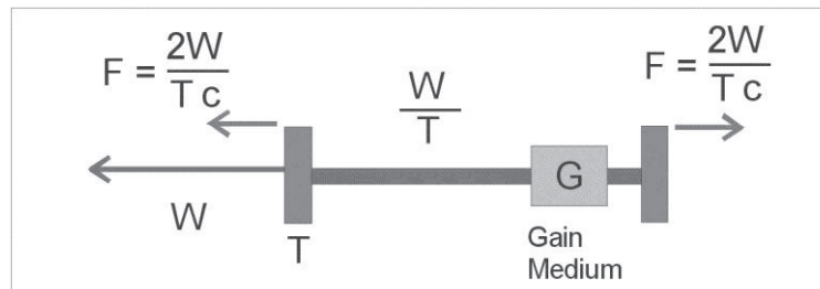
Fig. 3. Schematic diagram of the Photonic Laser Thruster (PLT), which is based on the active resonant optical cavity approach to photon thrust amplification.
