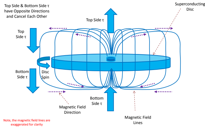
FIGURE 2. A possible (exaggerated) magnetic field structure over the superconducting toroidal disk.
