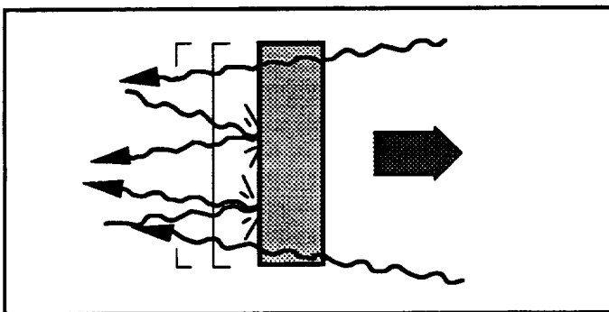
Fig. 2 Hypothetical Diode Sail Analogous to a diode or one-way mirror, space radiation passes through one direction and reflects from the other creating a net difference in radiation pressure.
