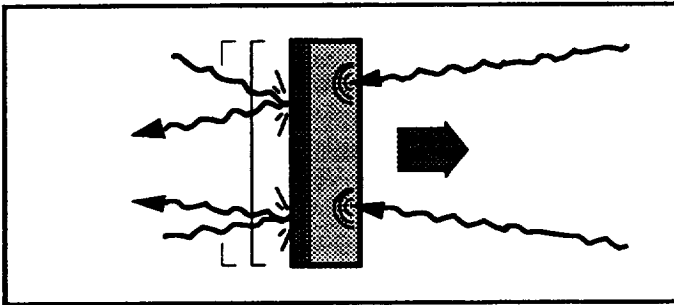
Fig. 1 Hypothetical Differential Sail Analogous to the principles of an ideal radiometer vane, a net difference in radiation pressure exists across the reflecting and absorbing sides.
