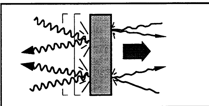
Fig. 3 Hypothetical Induction Sail Analogous to creating a pressure gradient in a fluid, the energy density of the impinging radiation is raised behind the sail and lowered in front of the sail to create a net difference in radiation pressure across the sail.
