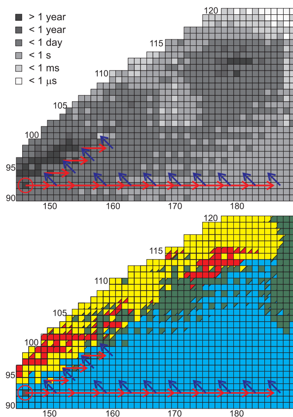
Figure 5. Half-lives (up) and decay modes (bottom) of nuclei in the upper part of the nuclear map. Schematic view of slow (terminated at the short-lived fission Fermium isotopes) and fast neutron capture processes with subsequent beta-minus decays are shown by the arrows.
