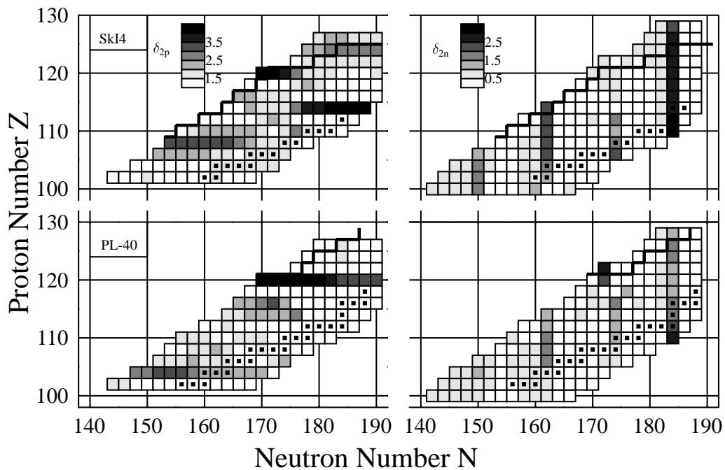
Figure 3. Grey scale plots of proton gaps (left column) and neutron gaps (right column) in the N-Z plane for deformed calculations with the forces SkI4 and PL- 40. Besides the spherical shell closures one can see the deformed shell closures for protons at Z = 104 (PL-40) and Z = 108 (SkI4) and the ones for neutrons at N = 162 for both forces.
