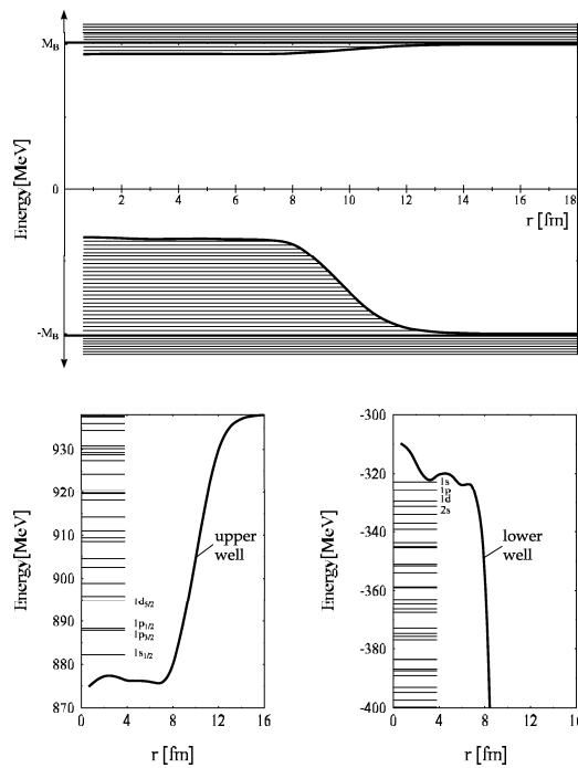
Figure 8. Baryon spectrum in a nucleus. Below the positive energy continuum exists the potential well of real nucleons. It has a depth of 50-60 MeV and shows the correct shell structure. The shell model of nuclei is realized here. However, from the negative continuum another potential well arises, in which about 40 000 bound particles are found, belonging to the vacuum. A part of the shell structure of the upper well and the lower (vacuum) well is depicted in the lower figures.
