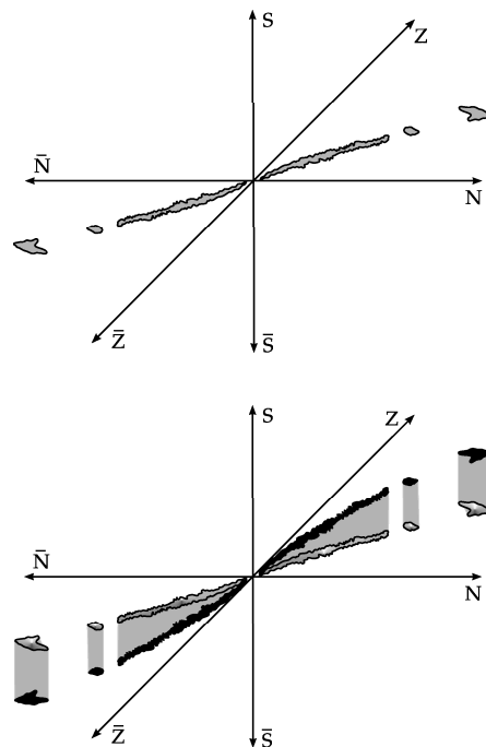
Figure 7. The extension of the periodic system into the sectors of strangeness S, \bar{S} and antimatter \bar{Z}\bar{N} . The stable valley winds out of the known proton (Z) and neutron (N) plane into the S and \bar{S} sector, respectively. The same can be observed for the antimatter sector. In the upper part of the figure only the stable valley in the usual proton (Z) and neutron (N) plane is plotted, however, extended into the sector of antiprotons and antineutrons. In the second part of the figure it has been indicated, how the stable valley winds out of the Z-N-plane into the strangeness sector.
