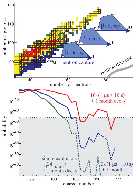
Figure 6. Schematic picture for multiple neutron irradiation of initial ^{238}\text{U} material (up) and probability for formation of heavy nuclei (bottom) in such process (one, three and ten subsequent explosions). Dotted line denotes the level of few atoms.
