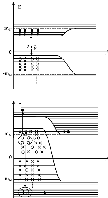
Figure 9. Due to the high temperature and the violent dynamics, many bound holes (antinucleon clusters) are created in the highly correlated vacuum, which can be set free during the expansion stage into the lower continuum. In this way, antimatter clusters can be produced directly from the vacuum. The horizontal arrow in the lower part of the figure denotes the spontaneous creation of baryon-antibaryon pairs, while the antibaryons occupy bound states in the lower potential well. Such a situation, where the lower potential well reaches into the upper continuum, is called supercritical. Four of the bound holes states (bound antinucleons) are encircled to illustrate a “quasi-antihelium” formed. It may be set free (driven into the lower continuum) by the violent nuclear dynamics.
