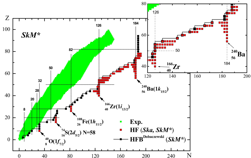
Figure 4. Fragment of the neutron drip line and elements (red squares) that are stable against one neutron emission [17]. One can see the formation of stability peninsulas along neutron magic numbers.
