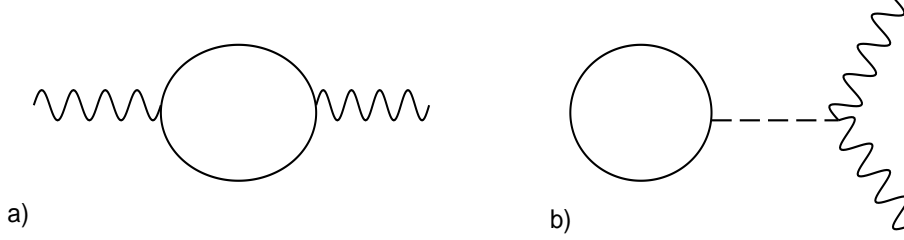
Figure 16: a) One-loop gauge coupling correction due to charged particles. b) Universal one-loop correction.
