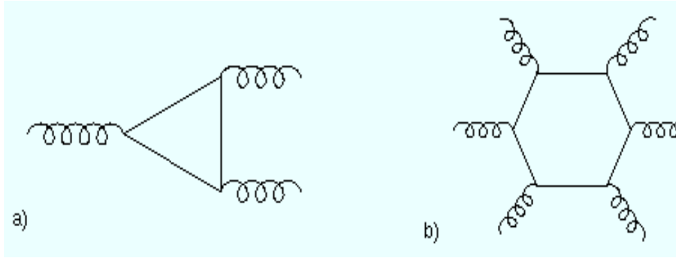
Figure 14: a) The anomalous triangle diagram in four dimensions. b) The anomalous hexagon diagram in ten dimensions.
