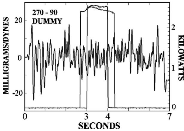
Fig. 13. The currents emulation test results obtained with the dummy circuit shown in Fig 12.
