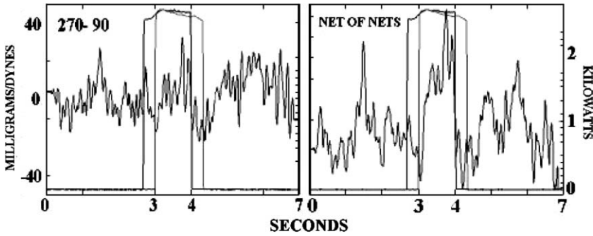
Fig. 10. The 270-90^\circ of relative phase for the reversed inductor polarity (left panel) and those results minus the unreversed 270-90 degrees data (right panel of Fig. 8) giving a “net of nets” for these relative phases of the inductor current and capacitor voltage.
