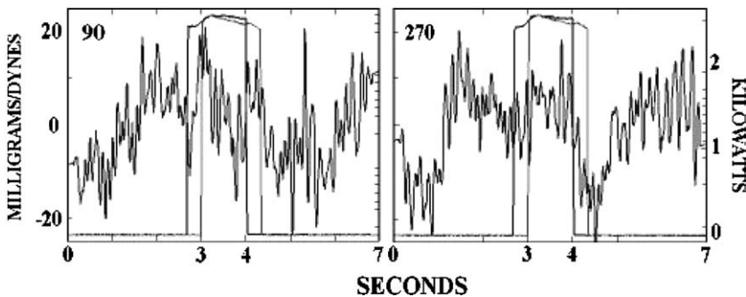
Fig. 9. The 90^\circ and 270^\circ of relative phase results obtained when the polarity of the current in the inductors was reversed at the plug in the Faraday cage.
