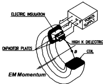
Fig. 3. A schematic diagram of one of H. Brito's toroidal flux capacitors.
