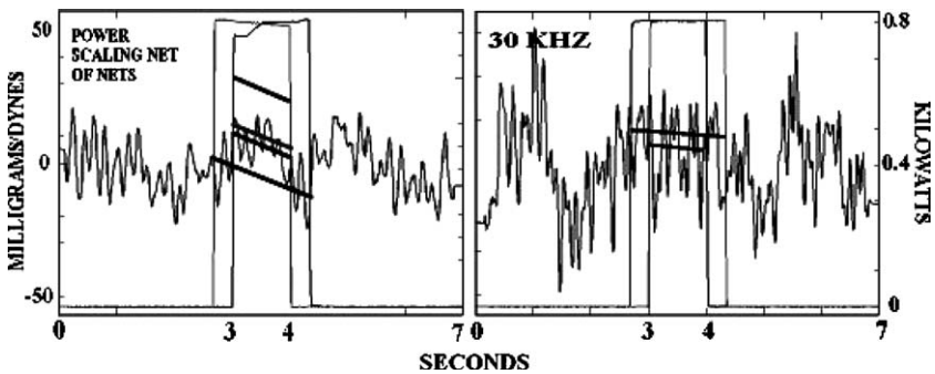
Fig. 14. The results for the power scaling test (left-hand panel) and frequency/power scaling test (right-hand panel). In both cases the line that roughly bisect the weight/thrust trace in the 3–4 s interval is that which corresponds to expected Mach effect behavior.
