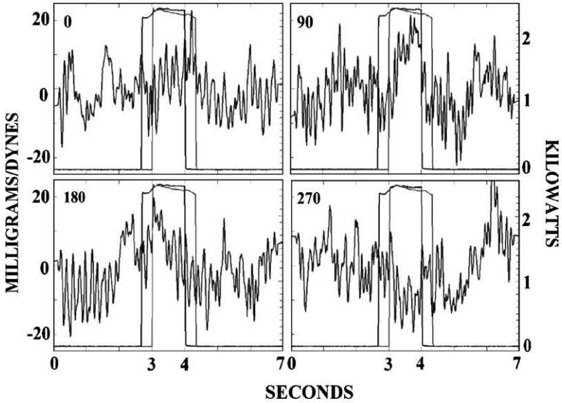
Fig. 7. Results (averages of about 200 cycles) for the four relative phase angles between the inductor current and capacitor voltage at high power (roughly 2.5kW amplitude power wave delivered to the capacitors).
