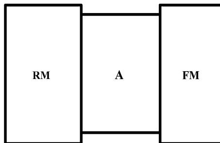
Fig. 1. A schematic diagram of a Mach effect “impulse engine” comprised of a reaction mass (RM), piezoelectric actuator (A), and a fluctuating mass (FM) element in which the Mach effect is driven.
