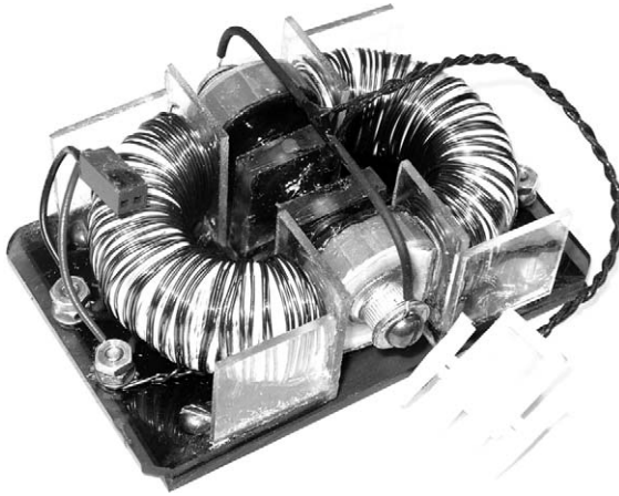
Fig. 4. The flux capacitor device used in this experiment comprised of two modified high voltage disk capacitors (center top and bottom) and a split toroidal inductor core on which coils are wound (left and right). Note the inductor circuit connector on the left that allows change of the inductor polarity close to the inductors.
