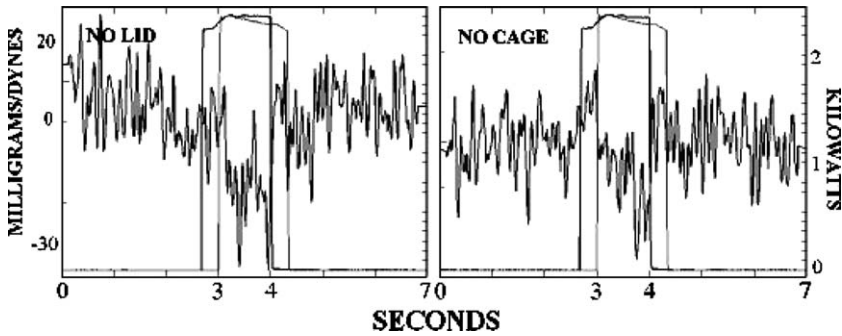
Fig. 11. The 270–90° of relative phase results obtained with part (no lid) or all (no cage) of the Faraday cage removed from the test chamber.
