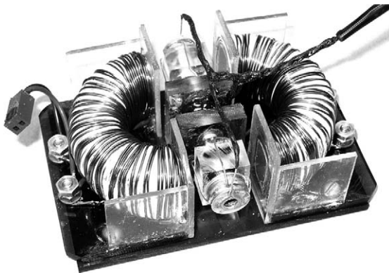
Fig. 12. The currents emulation test device used to insure that electromagnetic coupling to the environment could not be the cause of the signals seen in Figs. 7–11.
