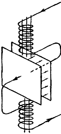
Fig. 2. A schematic diagram of a “flux” capacitor [after Corum, et al. (14) ] in which the material between the plates of the capacitor is subjected to an AC electric field and a perpendicular, high flux AC magnetic field produced by the inductors ranged above and below the capacitor in the drawing.
