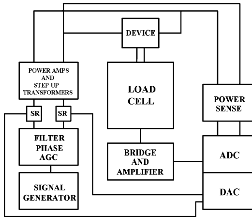
Fig. 6. A block diagram of the chief electrical and electronic circuits in the apparatus.
