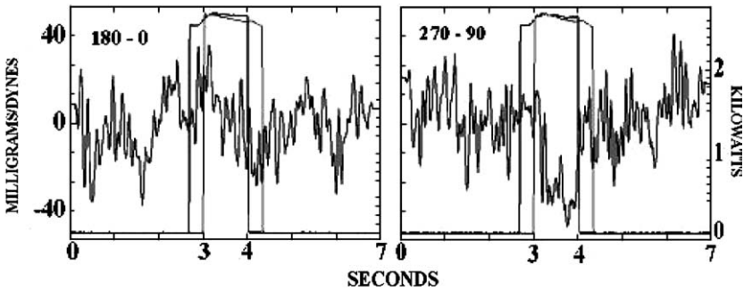
Fig. 8. Differenced results for 180-0° and 270-90° of relative phase between the inductor current and capacitor voltage. Note the prompt effect when both the inductors and capacitors are energized in the 270-90° data.
