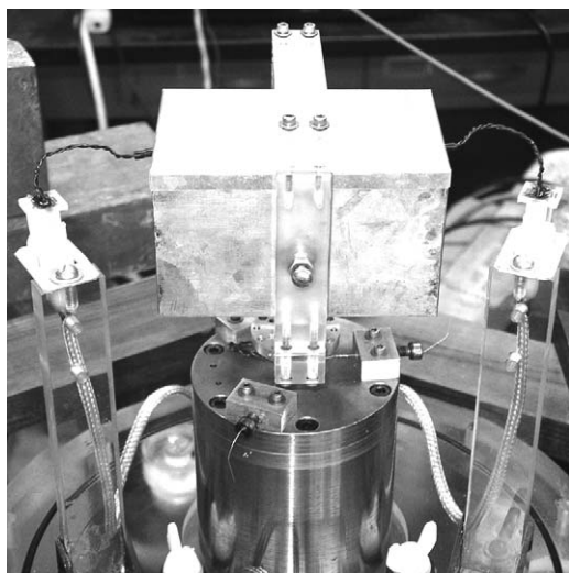
Fig. 5. The Faraday cage (steel box) mounted atop the thrust weight sensor (in the cylindrical steel shield at the bottom center).
