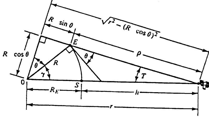
Figure 4.7: Earth satellite geometry, as explained in the text. Adopted from [15].
