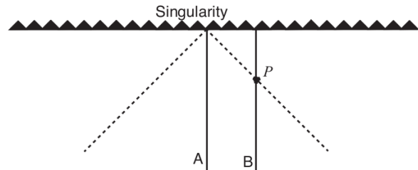
FIG. 2: The world lines of two observers, A and B, falling into a BKL singularity (the solid lines), and the particle horizon of observer A (dashed lines; a past light cone). Events outside the particle horizon can never influence observer A.
