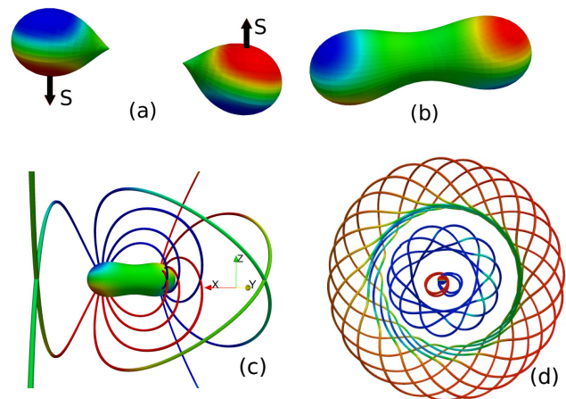
FIG. 9: (Color online.) The event horizons and vortex lines of spinning black holes, colliding head-on with transverse spins; from the simulation reported in [22]. (a) Horizon vortexes and spin directions just before merger. (b) Horizon vortexes just after merger, which retain their individuality. (c) Vortex lines linking horizon vortexes of same polarity (red to red or dark gray to dark gray; blue to blue or light gray to light gray). Lines are color coded by vorticity (different scale from horizon). (d) Sloshing of near-zone vortexes generates toroidal vortex loops (two shown here) composed of orthogonal vortex lines, traveling outward as gravitational waves; these are accompanied by intertwined tendex lines (not shown). The horizon, with attached vortex lines, is visible in the center. Figure adapted from [20]. See [23] for a movie of horizon vortexes for this simulation.
