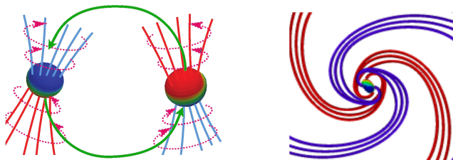
FIG. 10: (Color online.) Left: Schematic of vortex lines and horizon vortexes for two orbiting, spinning black holes about to merge. Right: Schematic of vortex lines of the remnant black hole just after merger, showing vortex lines extending to large distances; the entire pattern is rotating counterclockwise.
