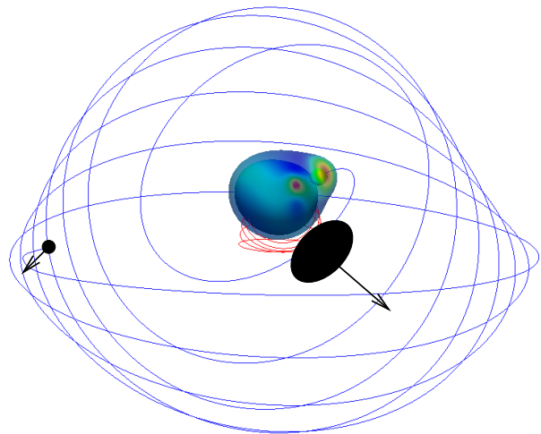
FIG. 13: (Color online.) The two thin curves are the trajectories of the centers of two black holes in a generic orbit; from a simulation presented in [30]. The mass ratio of the two holes is 6:1, and the dimensionless spins of the larger and smaller holes are S/M^2 = 0.91 and 0.3 , respectively (compared to the maximum possible spin S/M^2 = 1 ). The initial black hole positions are shown in black, and the initial spins are shown as arrows. The spins are initially oriented in generic directions, so that the orbital plane precesses. Shown also are the apparent horizons of both holes, and the common apparent horizon that encloses them, at the time the common apparent horizon first forms. The horizons are colored by the scalar Ricci curvature, which is approximately -2 times the horizon tendicity. See [31] for a movie of this simulation.
