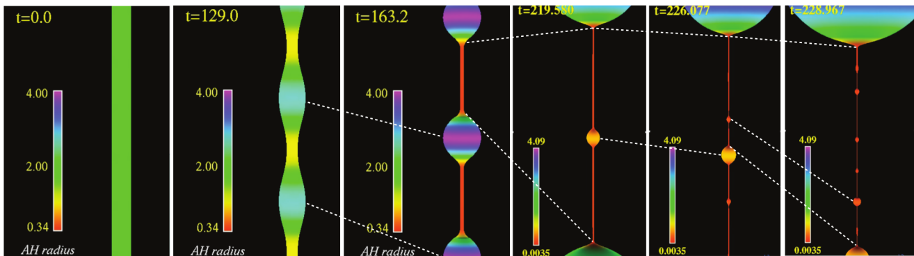
FIG. 5: (Color online.) A sequence of snapshots from a simulation of the geometrodynamical evolution of a black string in 5 spacetime dimensions, by Lehner and Pretorius [18]. Each snapshot is an embedding diagram of the black string’s event horizon: the horizon’s intrinsic geometry is the same as the intrinsic geometry of the depicted surface in flat space.
