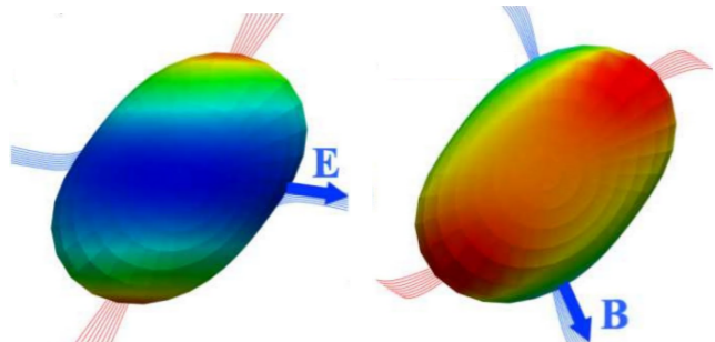
FIG. 12: (Color online.) Remnant horizon, shown in the xy plane, just after merger, for a superkick simulation tuned for maximum remnant recoil in the +z direction; from a simulation presented in [20]. The black hole and vortex/tendex structures rotate counterclockwise. Left: Colors show horizon tendicity; tendex lines are shown emerging from the strongest horizon tendexes. Right: Colors show horizon vorticity; vortex lines are shown emerging from the strongest horizon vortexes. Figure adapted from [20]. See [28] and [29] for movies of horizon vortexes and tendexes for this simulation.
