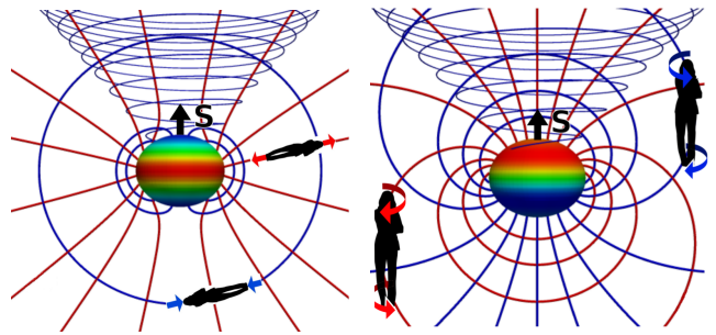
FIG. 7: (Color online.) Tendex lines (left panel) and vortex lines (right panel) near a spinning black hole. Lines with positive eigenvalues (tidal squeeze or clockwise twist) are shown blue or light gray, and lines with negative eigenvalues (tidal squeeze or counterclockwise twist) are shown red or dark gray. At each point in space there are three intersecting tendex lines and three intersecting vortex lines.
