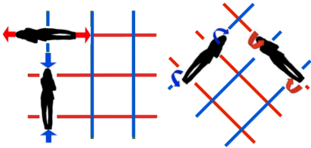
FIG. 8: (Color online.) Snapshot of vortex and tendex lines for a gravitational plane wave traveling into the page. Two orthogonal sets of tendex lines (left) are oriented 45 degrees with respect to two orthogonal sets of vortex lines (right). The third set of vortex (and tendex) lines is normal to the page, with zero vorticity (tendicity).
