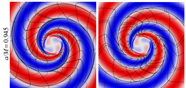
FIG. 11: (Color online.) Vortex and tendex structures for deviations from the final, Kerr black hole, at late times after the merger of a black-hole binary. These are the structures in the final hole’s equatorial plane, and the final hole has a dimensionless spin S/M^2 = a/M = 0.945 . Left: Perturbations generated by horizon vortexes—vortex lines (solid black for clockwise, dashed for counterclockwise), and vorticity of the dominant vortex at each point (colored blue or light gray for clockwise and red or dark gray for counterclockwise). Right: Perturbations generated by horizon tendexes—tendex lines (solid black for squeeze, dashed for stretch), and tendicity of the dominant tendex (blue or light gray for squeeze and red or dark gray for stretch). Adapted from Fig. 12 of [24].
