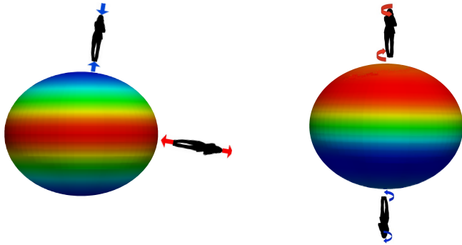
FIG. 6: (Color online.) A spinning black hole. Left: Colors represent horizon tendexity \mathcal{E}_{nn} . There is a positive (blue or light gray) tendex on each of the poles, and a negative (red or dark gray) tendex on the equator. Other (green or medium gray) regions have small tendexity. Right: Colors represent horizon vorticity \mathcal{B}_{nn} . There is a negative (red or dark gray) vortex on the north pole, and a positive (blue or light gray) vortex on the south pole. Other (green or medium gray) regions have small vorticity. The spin vector points out of the north pole.
