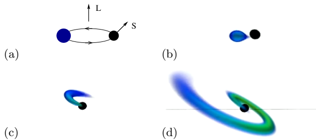
FIG. 14: (Color online.) Four successive snapshots of a collision between a black hole (black) and a neutron star (blue or gray), viewed edge-on in the initial orbital plane; from a simulation reported in [33]. (a) The initial black-hole spin S is inclined with respect to the initial orbital angular momentum L . (b) The black hole's tendexes begin to rip apart the neutron star. (c) Some of the matter falls down the black hole, but some remains outside the horizon. (d) The black hole's vortexes pull the remaining matter into the black hole's equatorial plane, forming a disk and a tidal tail. Figure adapted from [33]. See [34] for a movie of this simulation.
