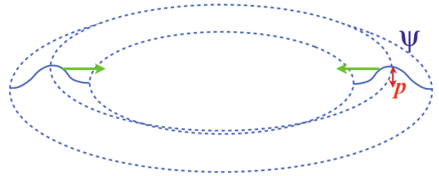
FIG. 1: The implosion of a scalar wave \Psi with amplitude p and a particular waveform.
