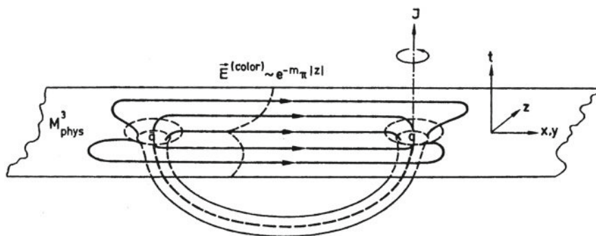
Fig. 15.1 Hadronic meson as “gluonic string” being trapped in a multiply connected Kerr–Newmann geometry
