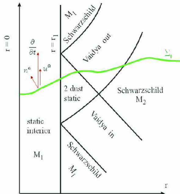
FIG. 1: (Color online) The static star, incoming and outgoing radiation zones, crossflowing null dust region and three exterior Schwarzschild domains. The normal vector n^a of the foliation leaf \Sigma_t is different from the fluid 4-velocity u^a . The foliation is chosen so that time evolution in the static star region proceeds in the direction of the fluid world-lines.
