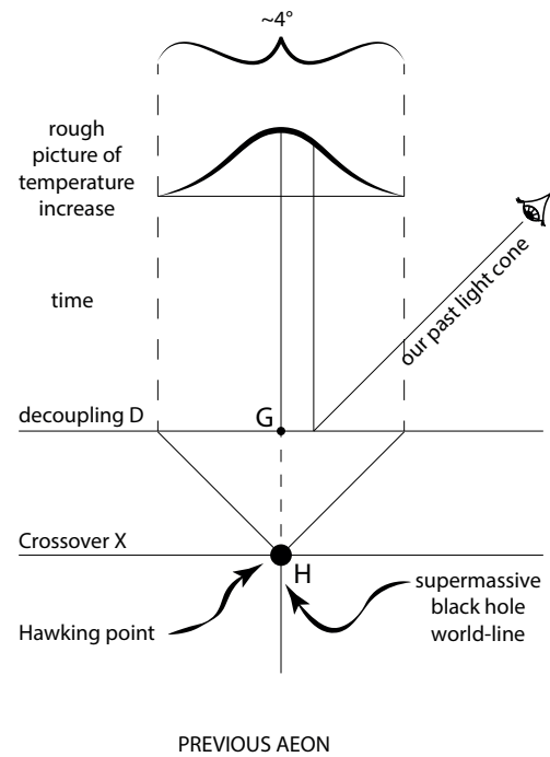
FIG. 1: A conformal diagram representing the effect of a highly energetic event occurring at the space-time point H. In CCC, H is taken to be a Hawking point, where virtually the entire Hawking radiation of a previous-aeon supermassive black hole is concentrated at H by the conformal compression of the hole's radiating future. The horizontal line at the bottom stands for the crossover surface dividing the previous cosmic aeon from our own and describes our conformally stretched Big Bang. In conventional inflationary cosmology, X would represent the graceful exit turn-off of inflation. In each case, the future light cone of H represents the outer causal boundary of physical effects initiated at H, and such effects can reach D only within the roughly 0.08 radian spread indicated at the top of the diagram.
