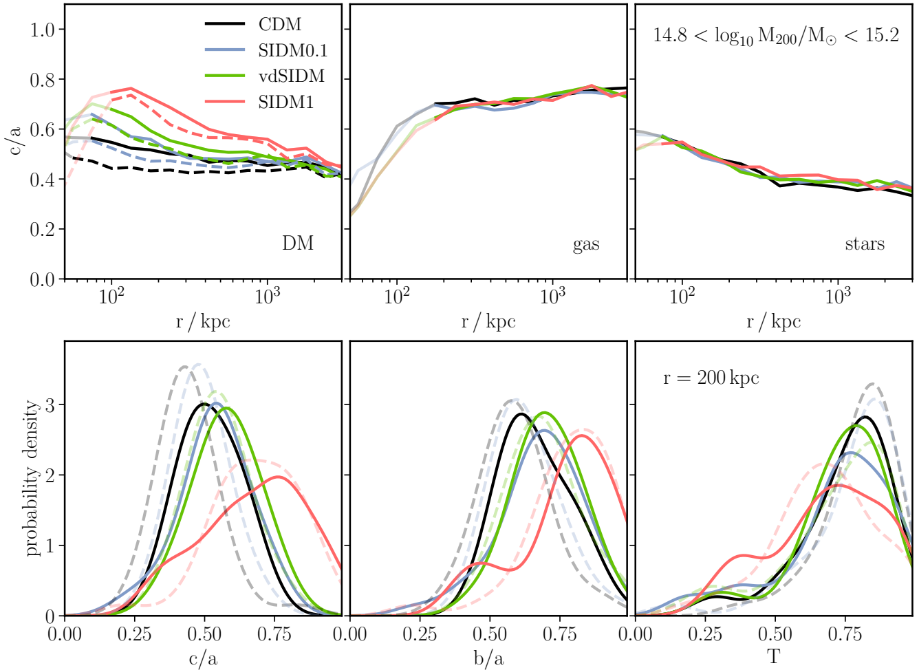
Figure 5. Top: the minor to major axis ratios for the DM, gas and stars from our different simulations at z = 0 , with the DM-only results represented by dashed lines. The lines shown are the medians from the \sim 40 haloes (per simulation) in the mass range 10^{14.8} - 10^{15.2} M_{\odot} , and become faded at radii where there are an insufficient number of particles to trust the shape measurements. Our definition of halo shape and the method used to calculate it is described in Section 4. While the DM halo becomes rounder (especially in the inner regions) with increasing cross-section, this is not obviously reflected in the shapes of either the gas or stars. Bottom: the distributions of DM axis ratios at r = 200 kpc, for the same haloes in the top panel. The triaxiality is defined by T = (a^2 - b^2)/(a^2 - c^2) , with values T \lesssim 1/3 and T \gtrsim 2/3 representing oblate and prolate distributions respectively. The DM-only lines in the bottom panels are faded to avoid distracting from the full physics results, not because we do not trust them.
