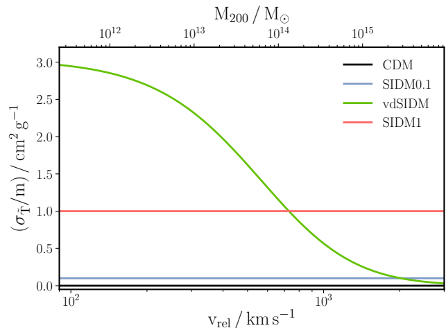
Figure 1. The momentum transfer cross-section for our four simulated DM models, as a function of the relative velocity between DM particles. This relative velocity has been roughly converted to a halo mass (along the top of the figure) using v_{\text{rel}} = \sqrt{GM_{200}/r_{200}} . The colour scheme used here for different DM models is continued throughout the rest of the paper.
