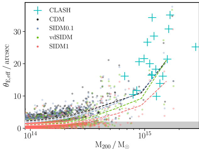
Figure 7. The effective Einstein radii of all simulated clusters with M_{200} > 9 \times 10^{13} M_{\odot} , for our four different DM models. The clusters were taken from the z = 0.375 snapshot, which was the lens redshift used, while the source redshift was z_s = 2 . The dashed lines show the median \theta_{E,\text{eff}} as a function of halo mass, with the points showing individual haloes. The grey shaded region indicates where we expect \theta_{E,\text{eff}} to be under-estimated due to the resolution of our simulations (discussed in Appendix C). The cyan crosses show CLASH clusters scaled to be at z = 0.375 (see Section 5.2.1).
