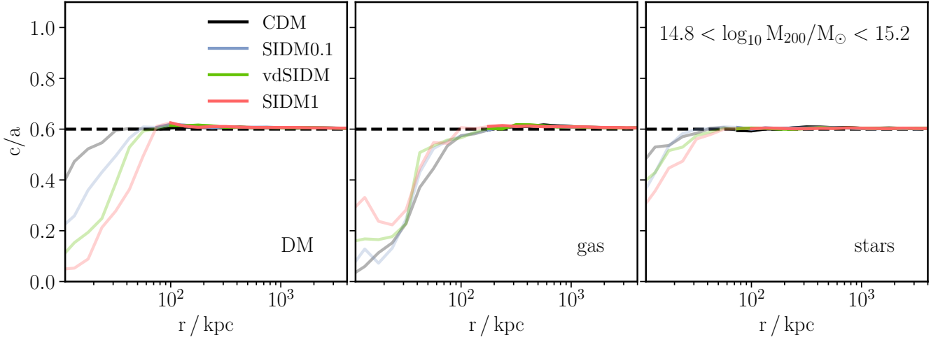
Figure B1. The median minor-to-major axis ratios of shuffle-stretched haloes, with a known true axis ratio of 0.6. The method used to derive halo shapes and generate the plot was identical to Fig. 5, but with the particle distributions from the simulated haloes altered following the procedure described in Appendix B. The lines are semi-transparent at radii where the median number of particles used for the shape measurement is less than 800. At small radii, where a small number of particles contribute to the shape measurement, the method is biased towards returning lower c/a than the true value. This bias is not present when more than 800 particles are used for the shape measurement.
