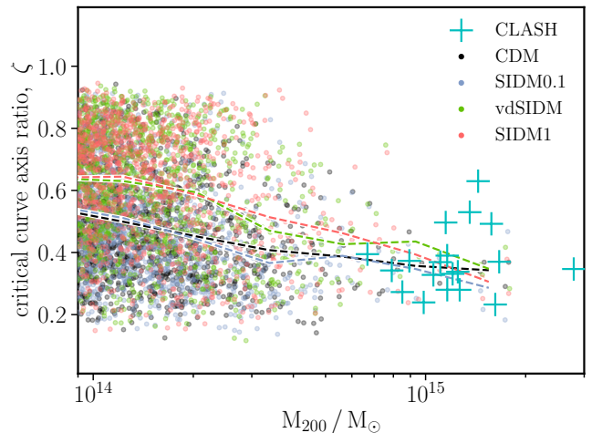
Figure 8. The minor-to-major axis ratios of our simulated clusters' critical curves, modelling them as ellipses (described in Section 5.2). The dashed lines are median axis ratios as a function of M_{200} for the different DM models. The cyan crosses show CLASH clusters scaled to be at z = 0.375 (see Section 5.2.1).
