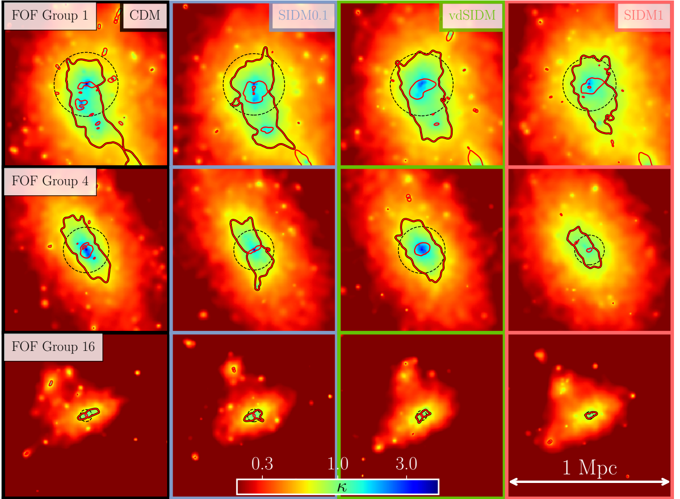
Figure 6. Convergence maps of the 1st, 4th and 16th most massive FOF groups in the BAHAMAS simulations, simulated with different SIDM cross-sections. The critical curves (with a lens redshift of z_1 = 0.375 and a source redshift z_s = 2 ) are plotted in red, with the largest tangential critical curve having a black outline. The dashed circles contain the same area as this largest tangential critical curve, and therefore represent the effective Einstein radius, \theta_{E,\text{eff}} . The scale of each panel is the same, covering a field of view of 1 Mpc in the lens plane, corresponding to approximately 3.2 arcmin.
