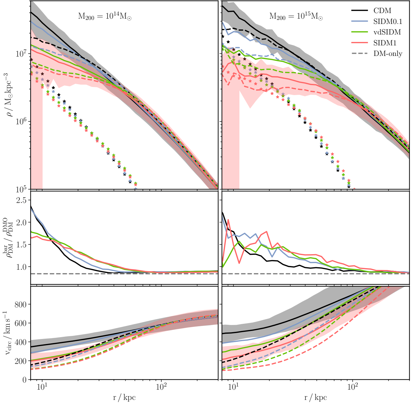
Figure 2. Top: stacked radial density profiles of our simulated clusters at z = 0 , with the left and right panels showing the results for clusters with M_{200} \approx 10^{14} and 10^{15} M_{\odot} respectively. The solid lines show the mean density profile of the DM from the full physics runs, while the dashed lines show the DM-only equivalents. The stars show the stellar density profile from the full physics runs. The black and red shaded regions show the 16-84th percentile ranges of DM profiles from the CDM and SIDM1 full physics simulations respectively. Middle: the mean DM density from simulations with full physics divided by the mean DM density from the corresponding DM-only simulations. The dashed lines show \Omega_{\text{DM}}/\Omega_{\text{m}} for our assumed cosmology. Bottom: the circular velocities, v_{\text{circ}} = \sqrt{GM(<r)}/r , for the total matter distributions from the same simulations/haloes as shown in the top panels.
