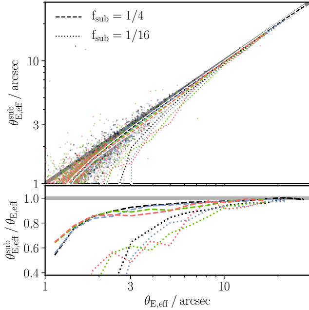
Figure C1. Top: the effective Einstein radius when using only every fourth or sixteenth particle from the simulations, versus the result using all the particles. The points show individual haloes when using every fourth particle, with the dashed lines the median relations (binned by \theta_{E,\text{eff}} when not subsampling). The dotted lines show the median relations when only a sixteenth of the simulation particles are used. The colours are for the different cross-sections as used throughout the rest of this paper. Bottom: the median lines from the top panel expressed as a relative value, showing the fractional bias in \theta_{E,\text{eff}} when subsampling.
