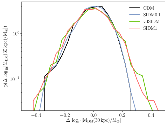
Figure 4. The PDF of \Delta \log_{10} [M_{\text{DM}}(30 \text{ kpc})/M_{\odot}] , for all haloes with 14.0 < \log_{10} [M_{200}/M_{\odot}] < 14.8 . \Delta \log_{10} [M_{\text{DM}}(30 \text{ kpc})/M_{\odot}] is defined for each halo as the difference in \log_{10} [M_{\text{DM}}(30 \text{ kpc})/M_{\odot}] between that halo and the corresponding median line shown in Fig. 3.
