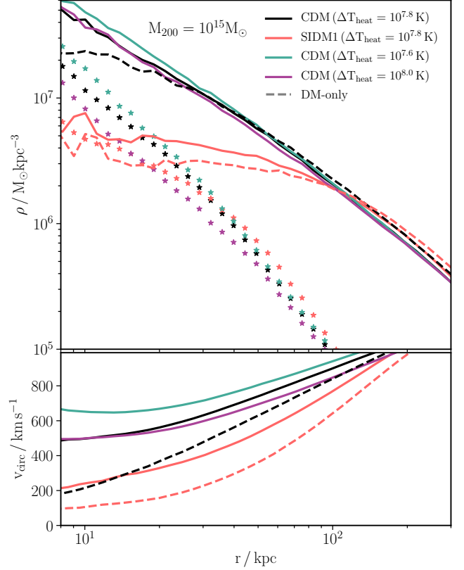
Figure A1. The same as the density and circular velocity panels from the right column of Fig. 2 but plotting only CDM and our largest SIDM cross-section, and additionally showing the density profiles of two additional CDM models with different AGN heating temperatures. While the changes to the stellar density induced by changing DM model or changing subgrid physics parameters are comparable, the DM density profile is more sensitive to the DM model than to changing \Delta T_{\text{heat}} .
