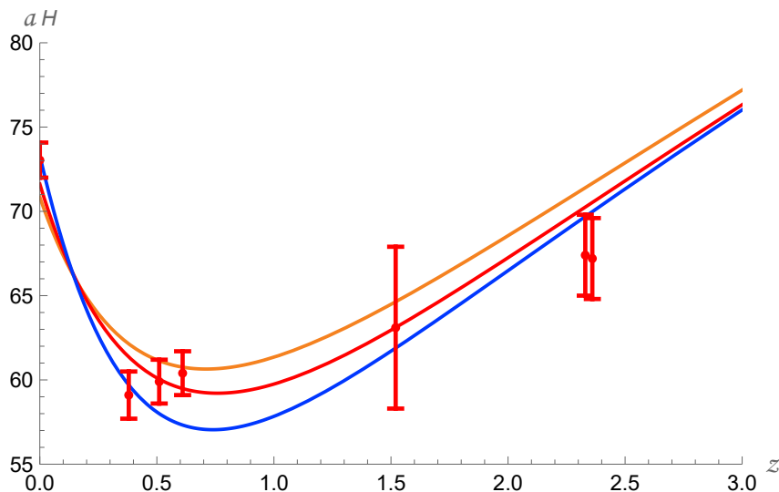
Figure 5. The graphs for H(z)/(1+z) for the three models using the values of H_0 from table 4. Orange graph corresponds to f_{\text{ds-model}} , blue graph to the f_{\text{mod-model}} and red graph to the f_{\text{gcdt-model}} .
