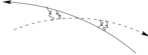
Fig. 3. Schematic representation of two intersecting branes and the open strings which are attached to both of them. They lead to an anti-align of the two branes.
