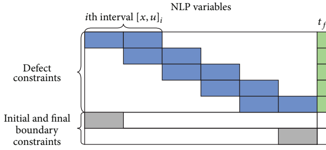
FIGURE 4: Jacobian structure for third-order Gauss-Lobatto method.
