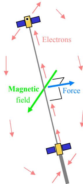
Figure 1. Electrodynamic Loop and Force
