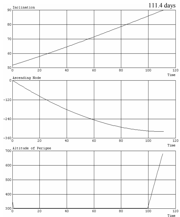
Figure 3. Orbit Transfer, ISS to Polar, Calculated by Navigation Tool
