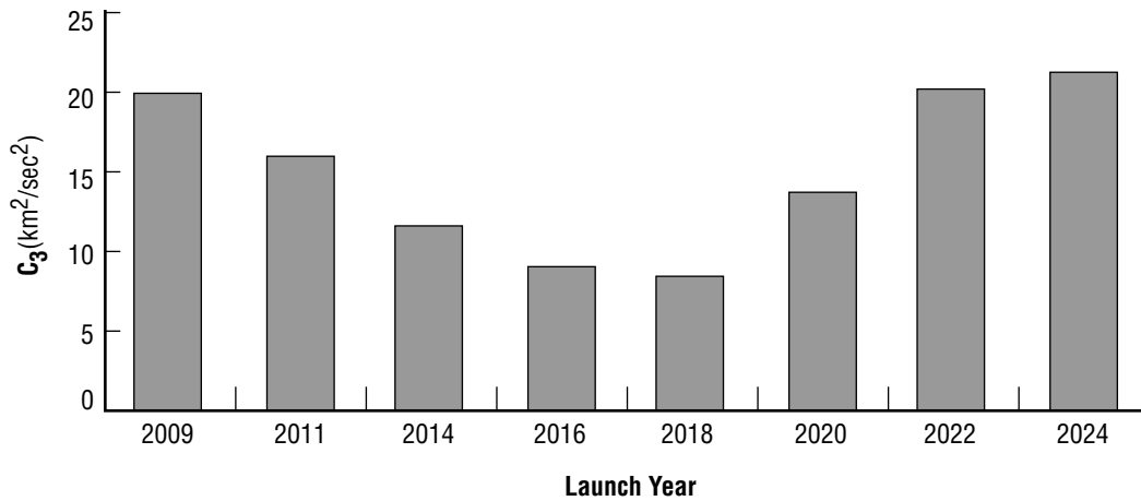
Figure 8. Piloted optimal departure energies, 2009–2024.
