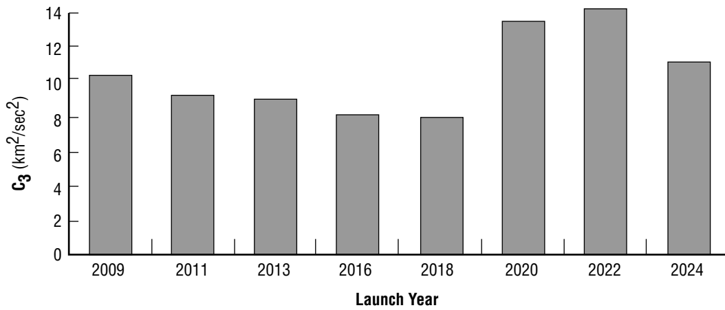
Figure 5. Cargo mission departure energies, 2009–2024.
