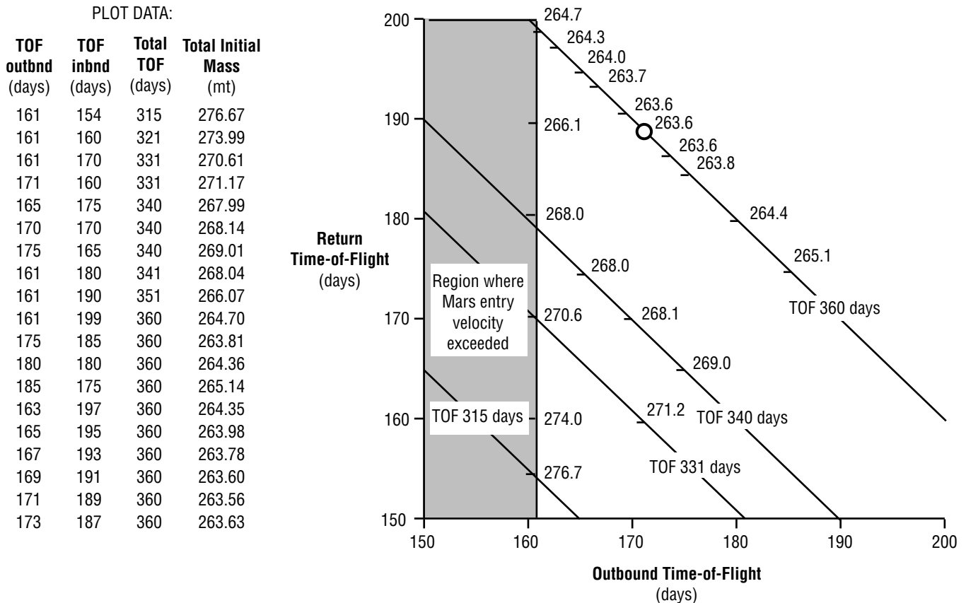
Figure 10. 2014 time-of-flight trade studies.
