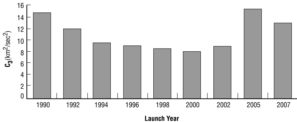
Figure 7. Cargo mission departure energies, 1990–2007.
