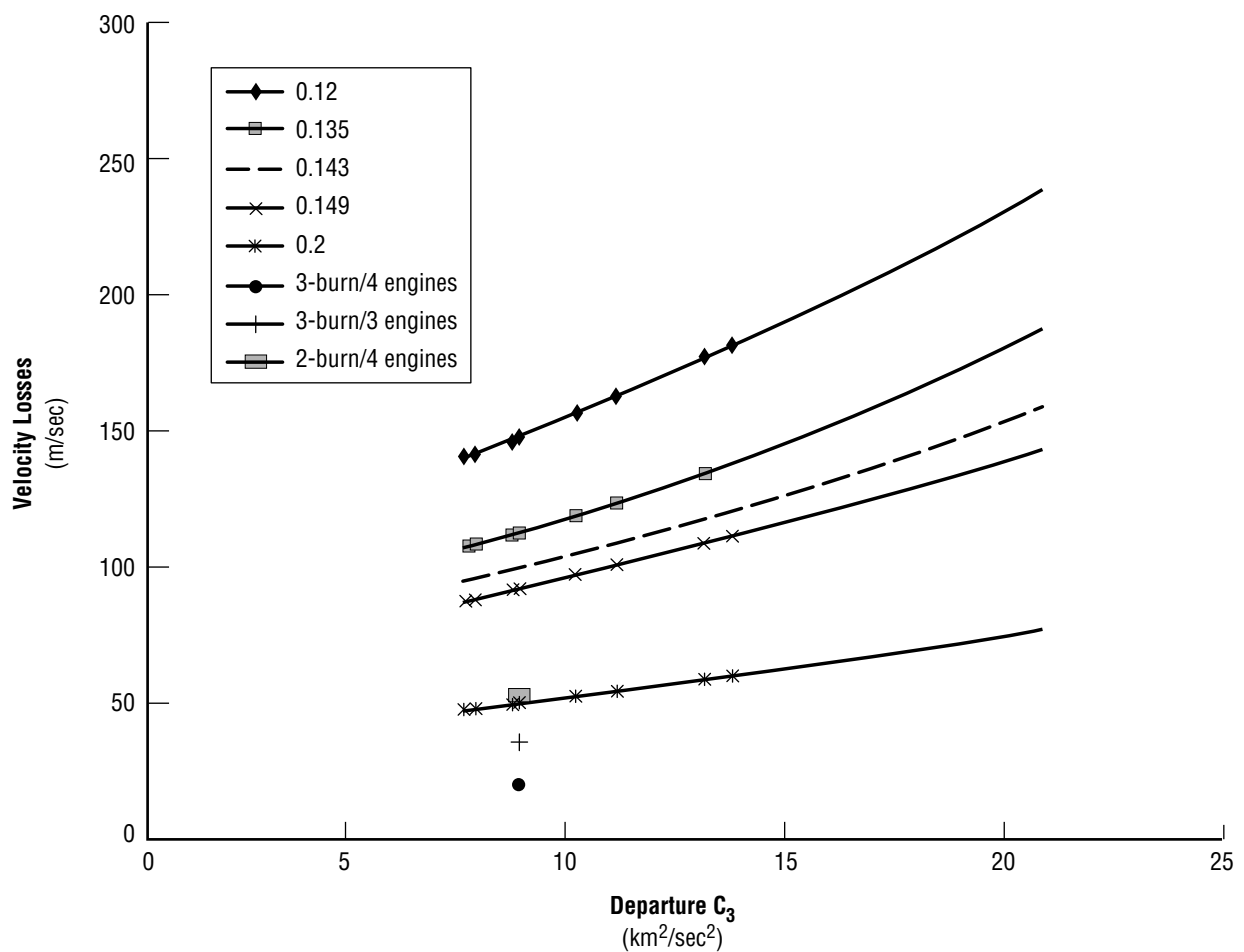
Figure 11. Velocity losses at various T/W ratios.
