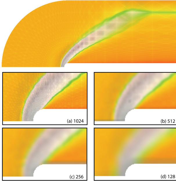
Figure 4. The Blunt Fin dataset rendered into a 1024^2 image at (a) full quality and upsampled from (b) 512^2 , (c) 256^2 , and (d) 128^2 using our technique.
