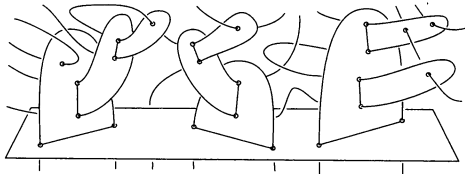
Fig. 2. Part of a Whitney tower in 4-space.
