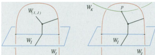
Fig. 6. Local pictures of the trees associated to a Whitney disk W_{\langle I, J \rangle} , and an intersection point p \in W_{\langle I, J \rangle} \cap W_K .
