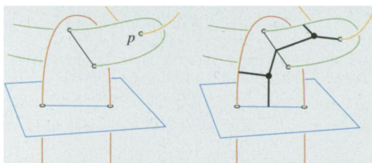
Fig. 3. An unpaired intersection-point p among local sheets in a Whitney tower (Left), and its associated tree (Right).
