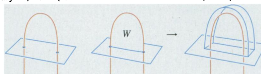
Fig. 1. (Left) A canceling pair of transverse intersections between two local sheets of surfaces in a 3-dimensional slice of 4-space. The horizontal sheet appears entirely in the “present,” and the red sheet appears as an arc that is assumed to extend into the “past” and the “future.” (Center) A Whitney disk W pairing the intersections. (Right) A Whitney move guided by W eliminates the intersections.
