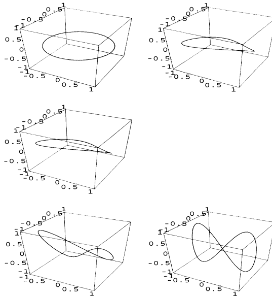
FIG. 3.5. Examples of projections of G(S^1) onto 2-dimensional linear subspaces of \mathbb{R}^3 . The top row of the figure shows two invertible projections. The center image is of a projection taken from the boundary of \bar{\Sigma} . The bottom row of the figure shows two noninvertible projections taken from within \Sigma .
