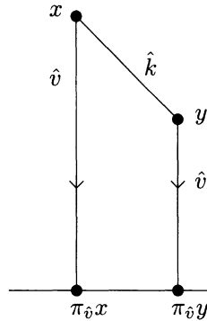
FIG. 3.1. The projection of the data along direction \hat{v} .
