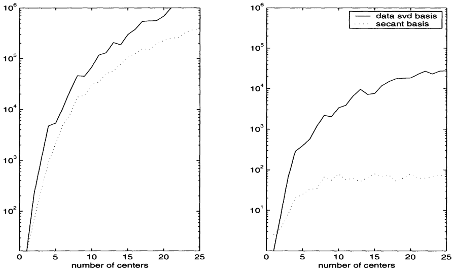
FIG. 5.4. \alpha = 84 . Left: Condition number of the interpolation matrix as a function of the number of centers in the radial basis function approximation. Right: Complexity of the RBF approximation as computed by (5.10).
