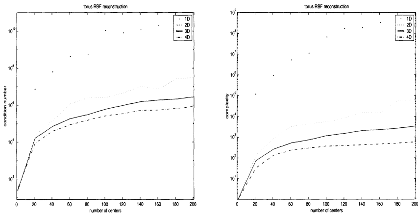
FIG. 5.5. \alpha = 87 . Left: Condition number of the interpolation matrix as a function of the number of centers in the radial basis function approximation. Right: Complexity of the RBF approximation as computed by (5.10).
