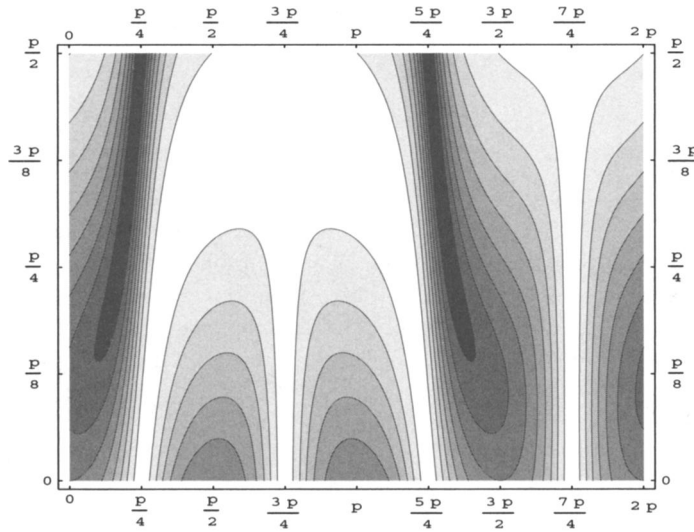
FIG. 3.6. Contour plot of the distance, d , between points on the great circle described in the text and points on the boundary of \tilde{\Sigma} . The abscissae parameterize the position on the boundary and the ordinates parameterize the position on the great circle. The darker the shade the smaller the value of d .
