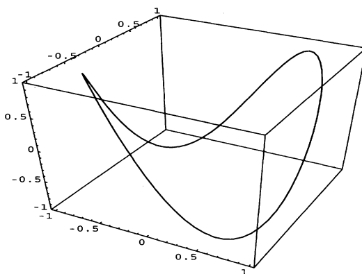
FIG. 3.2. The image of S^1 under the action of G .
